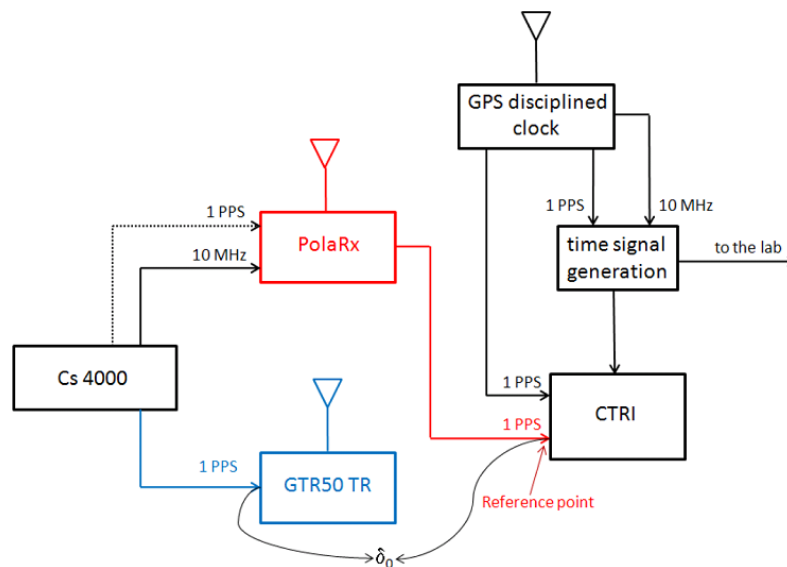
Figure 1. Scheme of time signal generation and remote comparison setup (red) at CERN and LNGS, with additional temporarily installed travelling equipment (blue).
