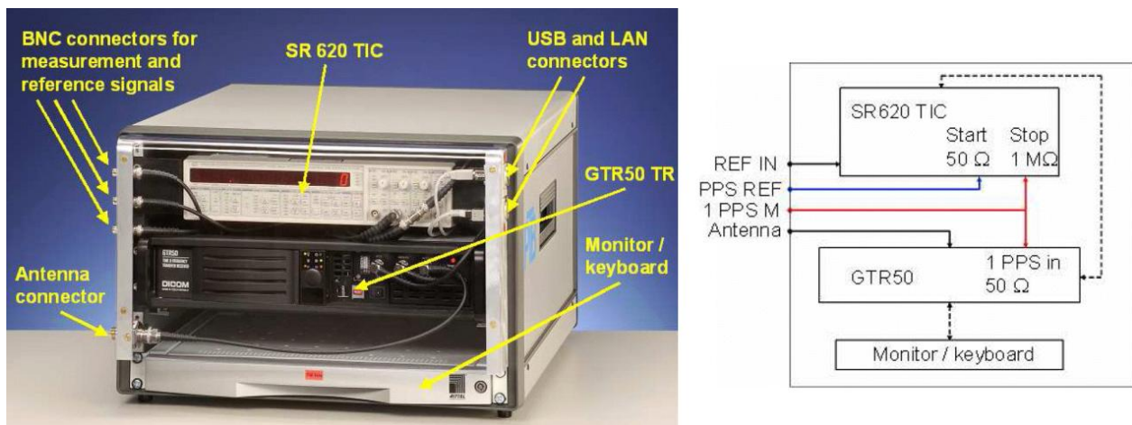
Figure 2. PTB's calibration set-up.
