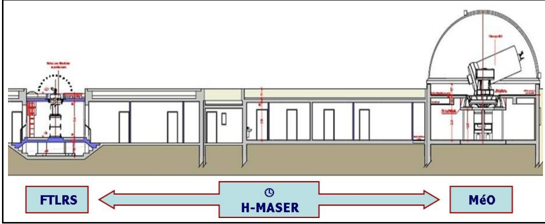
Figure 3. Common-clock time transfer between MeO and FTLRS in zero-baseline configuration at the OCA.
