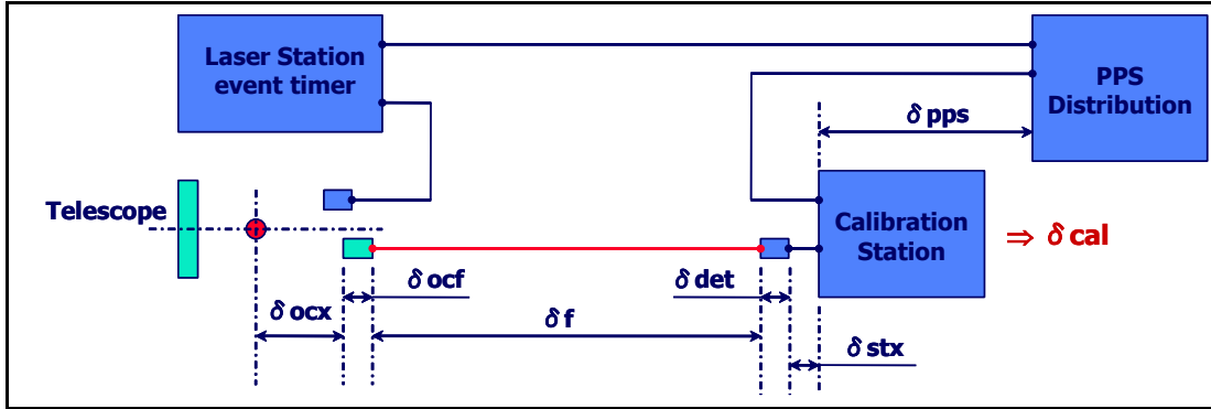
Figure 4. Experimental setup for the calibration of the propagation delay between the local time reference and the laser station time reference.
