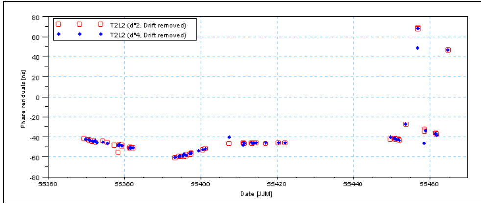
Figure 8. T2L2 ground-to-ground time transfer: Comparison of the two solutions, unique fourth-order polynomial on the whole pass, or sliding second-order polynomial on 30 s (same quadratic drift removed on the two data sets).
