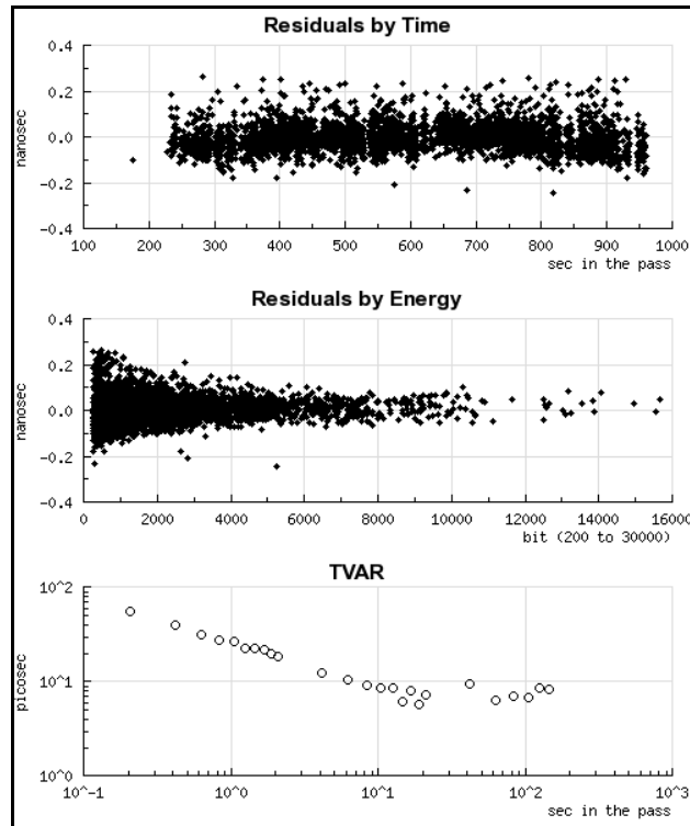
Figure 2. T2L2 Web site: Example of ground-to-space time transfer results (MeO station, Grasse, France, 03/09/2010 23h23-23h40 UTC).
