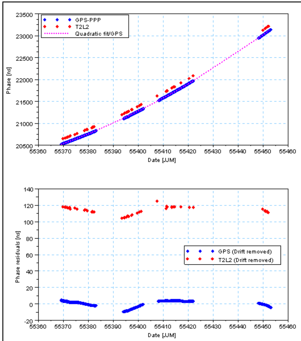
Figure 10. Ground-to-ground time transfer between Paris and Grasse: T2L2 and GPS solutions (top), T2L2 and GPS residuals (same quadratic drift removed on the two data sets, bottom).
