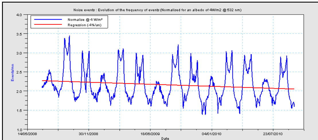
Figure 1. Frequency of “noise” events recorded by T2L2: Short-term variations are induced by the evolution of the attitude of the space vehicle.
