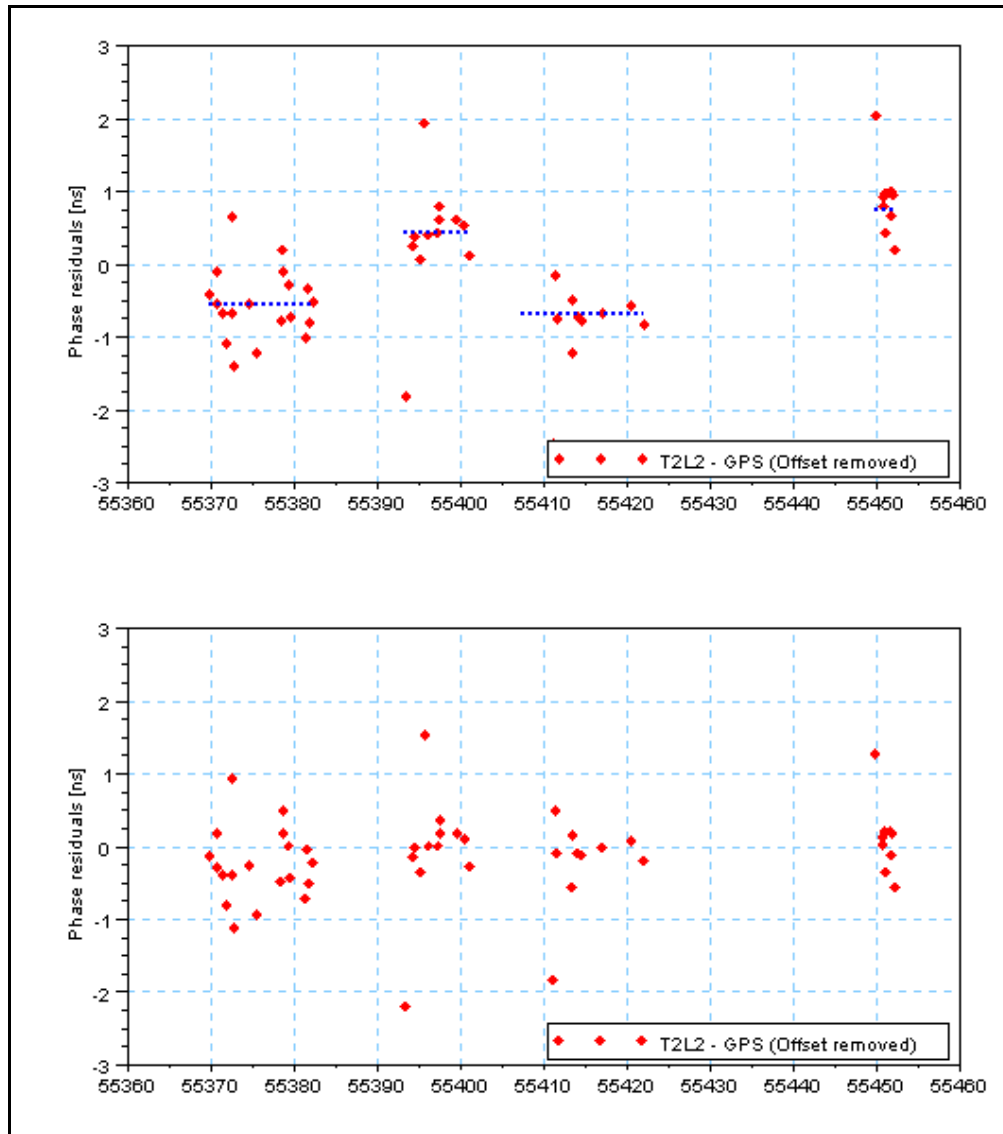
Figure 11. Difference between T2L2 and GPS ground-to-ground time transfer (115 ns offset removed) before (top) and after (bottom) resolution of the “wide lane” ambiguity thanks to T2L2 data.
