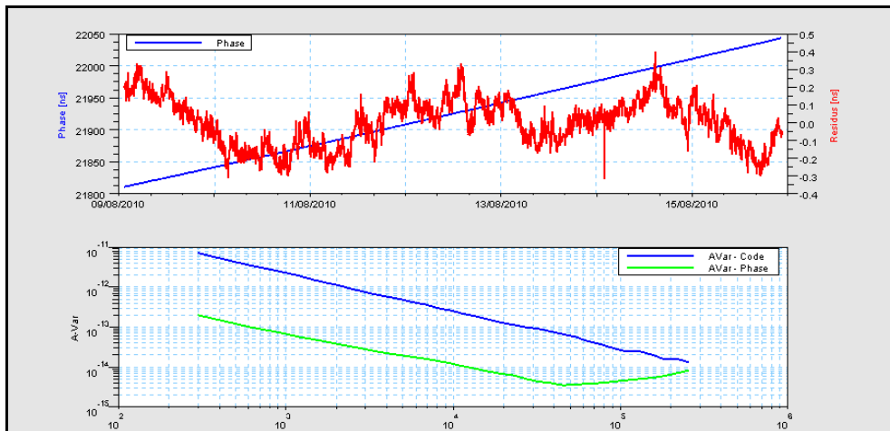
Figure 9. Typical performances of Carrier-Phase Time Transfer/Precise Point Positioning method with ambiguity resolution on zero-difference measurements (OP/Z12-T vs. OCA/GTR50 link, H-masers).
