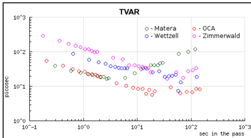
Figure 7. Ground-to-space time transfer stability (T-Var): Zimmerwald (02/09/2010 @ 00h36), Grasse (03/09/2010 @ 23h23), Matera (05-09-2010 @ 01h49), Wettzell (06/09/2010 @ 16h44).
