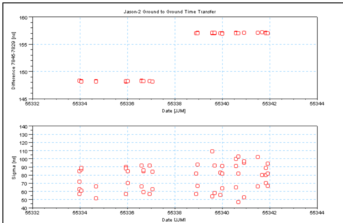
Figure 5. Ground-to-Ground time transfer between the two laser stations MeO (7845) and FTLRS (7829), May 2010.
