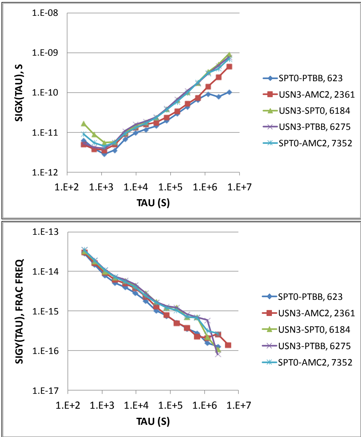
Figure 6. Allan and time deviation of (\text{Clk 1} - \text{Clk 2})_{\text{USNO rapid}} - (\text{Clk 1} - \text{Clk 2})_{\text{IGS rapid}} 1 November 2009-29 October 2010. The distance of each link is given in kilometers. PTBB is located in Braunschweig, Germany; AMC2 is located in Colorado Springs, Colorado.
