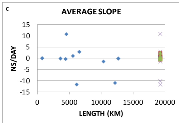
Fig 8c. Average frequency differences between USNO ultra-rapid and IGS rapid time-transfer estimates for time links originating at USN3.
