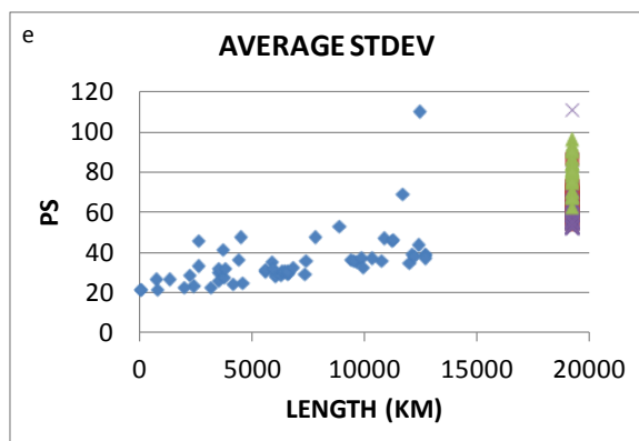
Fig 4e. Average standard deviation of linear fit between USNO and IGS rapid time-transfer estimates for time links originating at USN3.
