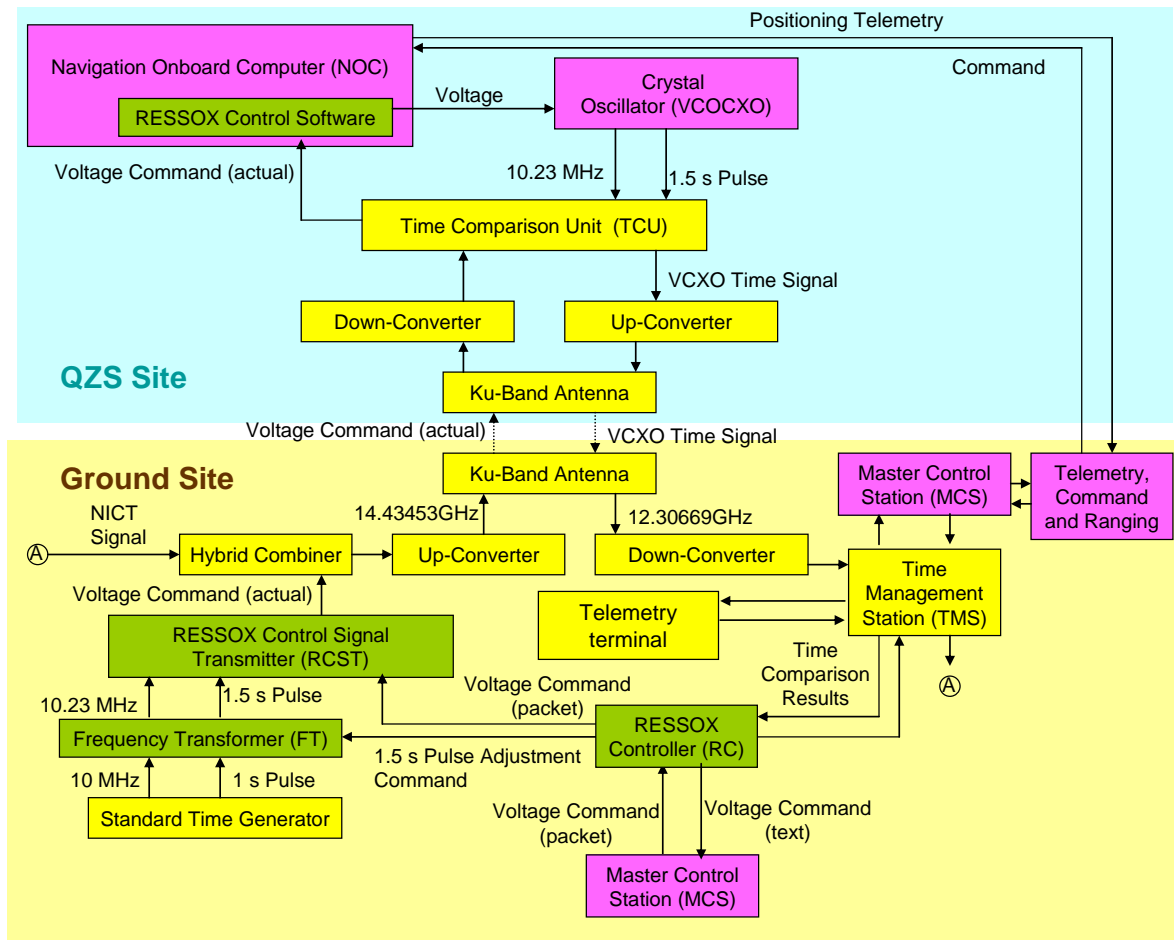
Fig. 3. System diagram of Experiment Two using QZSS.
