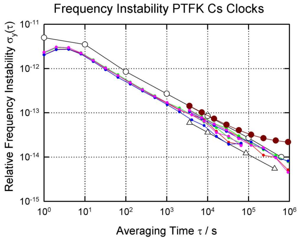
Figure 11. Instability of RCE cesium clocks. Large white circles: specification of 5071A clock type; large dark red circles: requirement for RCE system; white triangles: PTB's primary frequency standard CS2 (used as reference); small red, magenta, blue, and green circles: four RCE cesium clocks under test. The 5071A cesium clocks meet the manufacturer specifications; the \sigma_y(\tau) values lie between the primary clock CS2 and the RCE requirement.
