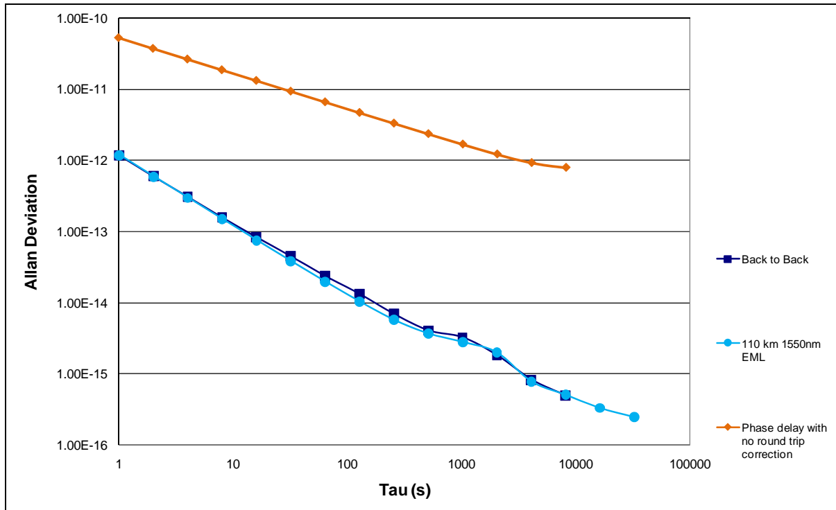
Figure 3. Allan deviation plot comparing: (1) a Back to Back measurement \blacksquare (2) a measurement using thermally controlled EMLs at 1550 nm and a 110-km fiber link \bullet and (3) a one-way transfer of an LO phase signal over 110 km with no round-trip correction \blacklozenge .
