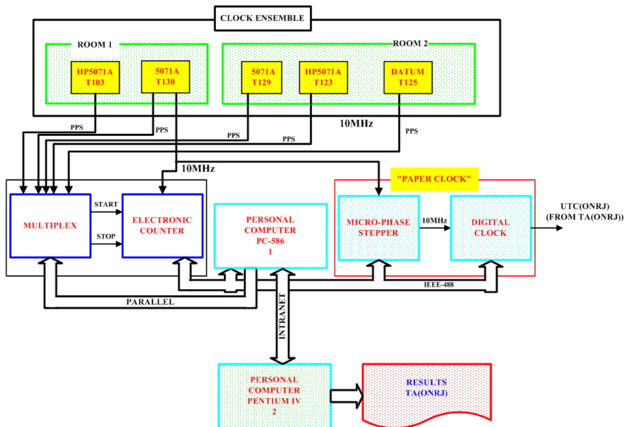
Figure 2. Block diagram of ONRJ time scale.
