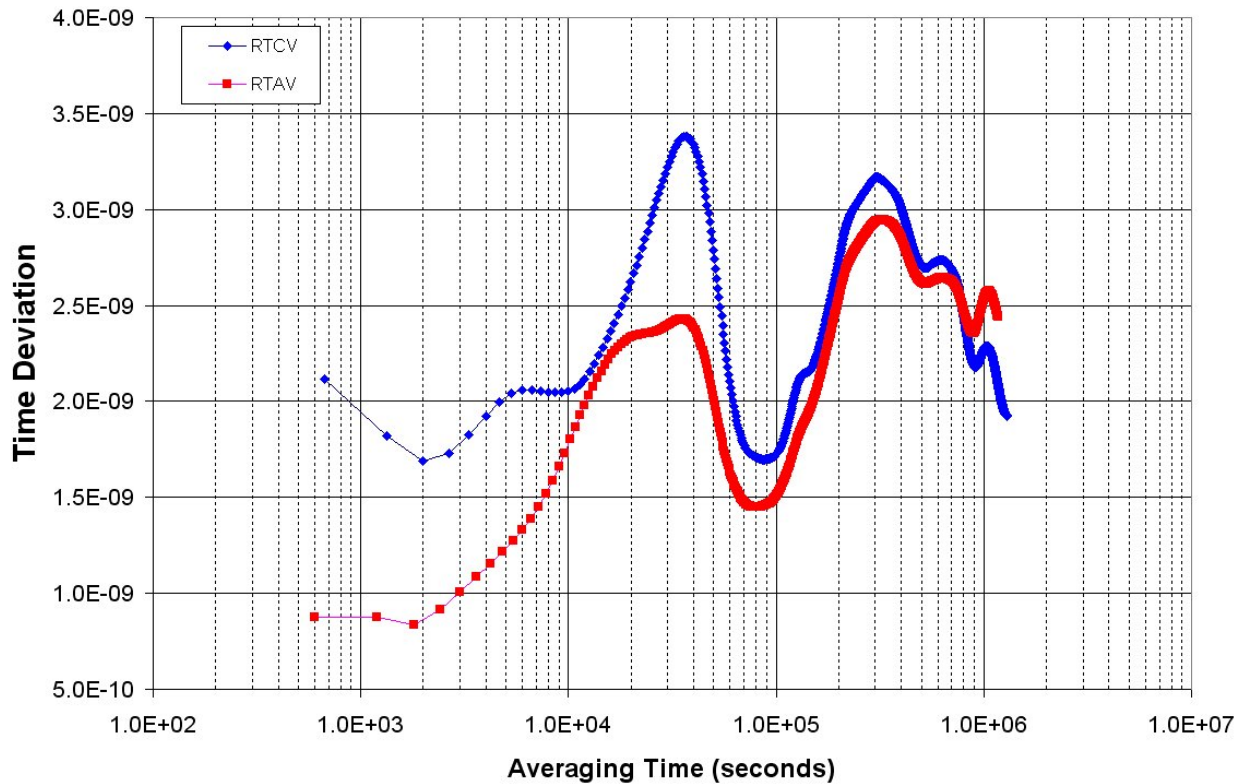
Figure 5. TDEV graph comparing the RTCV and RTAV methods.
