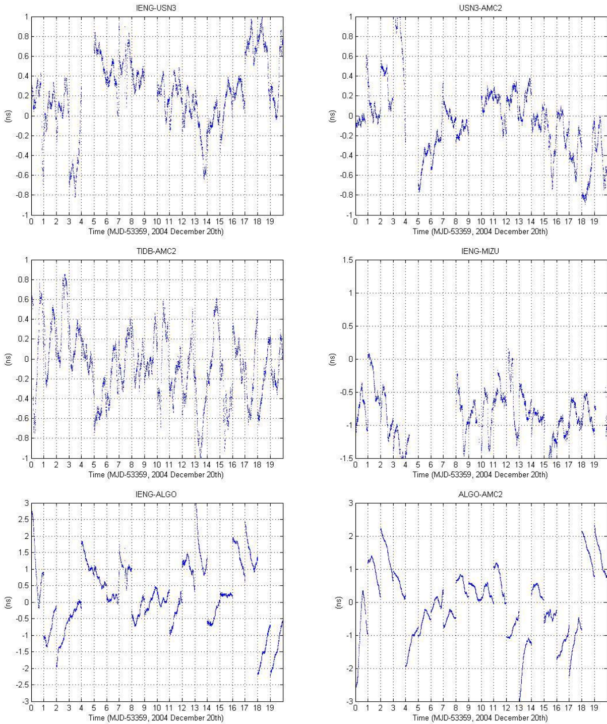
Figure 6. Double differences between RT estimates and IGS Final clock products for six selected baselines, for the period from December 20 th , 2004 (MJD 53359) to January 8 th , 2005 (MJD 53378).
