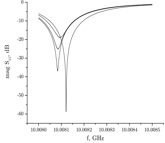
Fig. 9. Measured data of |S_{11}| at 10 GHz for different values of the variable phase shifter shown in Fig. 8.
