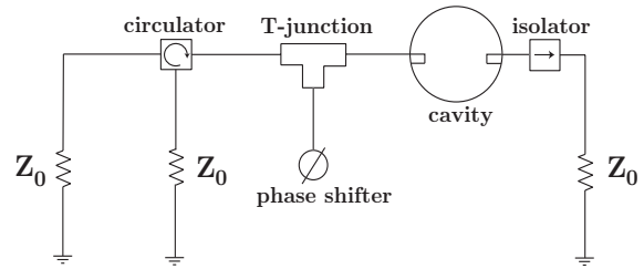
Fig. 1. Simplified diagram of the cavity circuit with input matching. Z_0 is the system's characteristic impedance.
