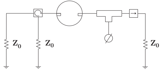
Fig. 8. Simplified diagram of cavity circuit with output matching. Z_0 is the system's characteristic impedance.
