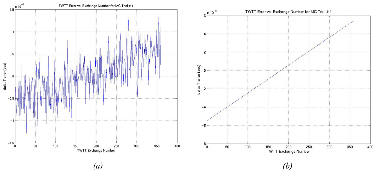
Figures 1(a) and 1(b). Error between actual clock offsets and measured offsets for transfers between NIST and the ISS with (a) modem noise included and (b) modem noise not included.
