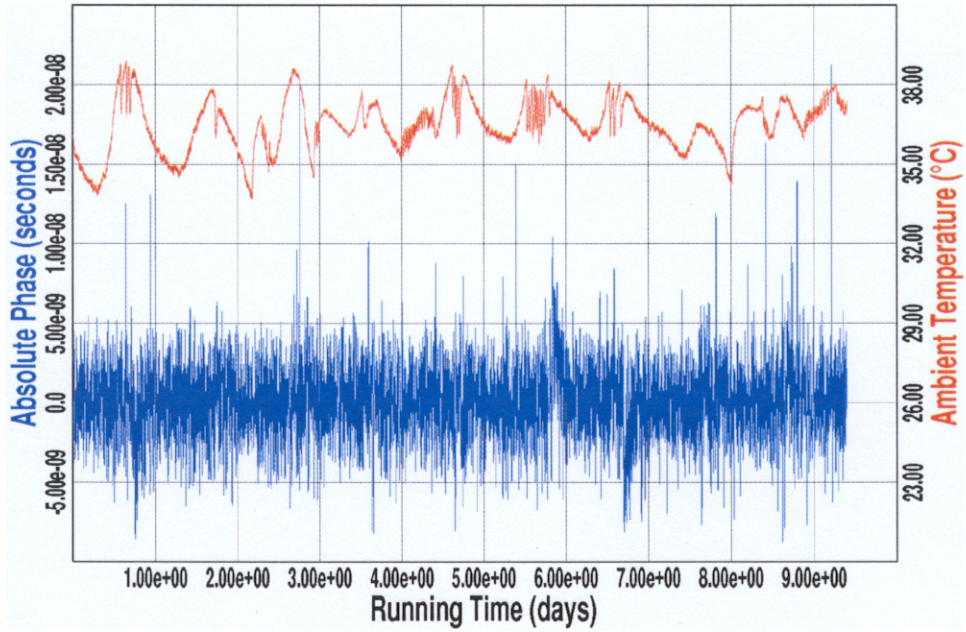
Figure 4 – GPS-Disciplined Rubidium Residuals 14-24 Nov. 2001
