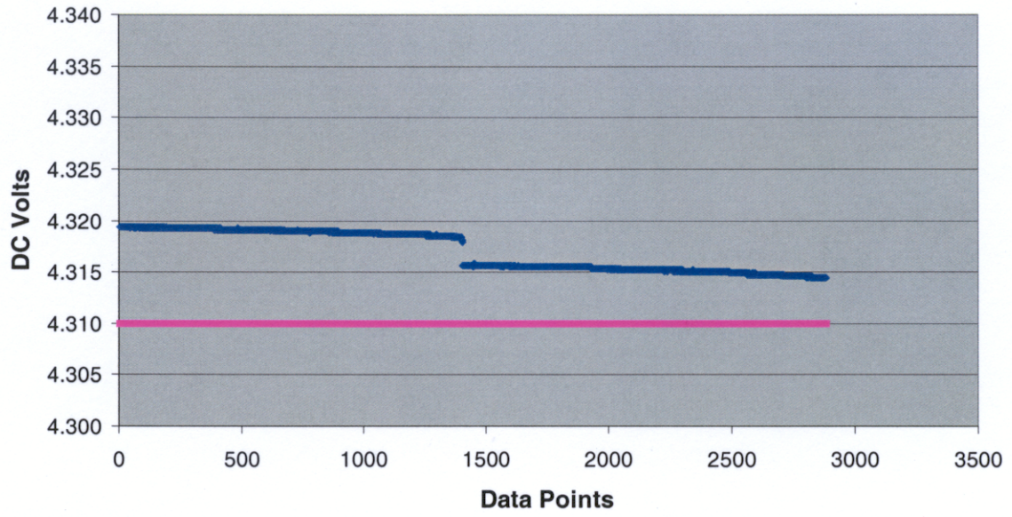
Figure 1. Telemetry Example.
