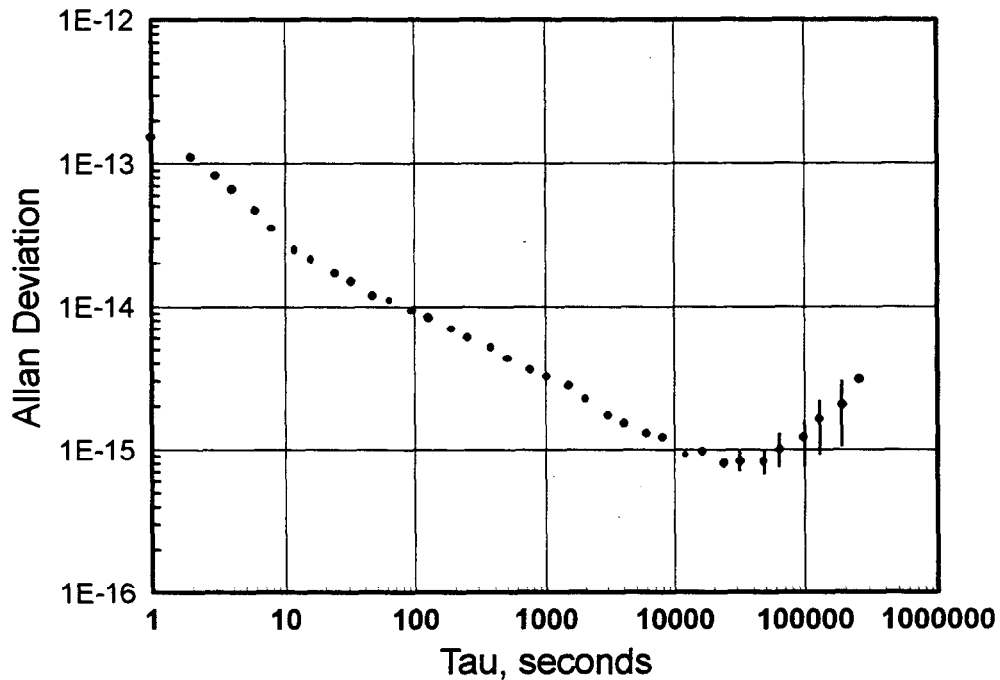
Figure 2: The Allan Deviation of the multi-pole trapped ion standard verse a SAO hydrogen maser. The slope of 1 \times 10^{-13} / \tau^{1/2} is expected as a result of using a H-maser as the local oscillator. The stability beyond 30,000 seconds is limited by the reference H-maser.
