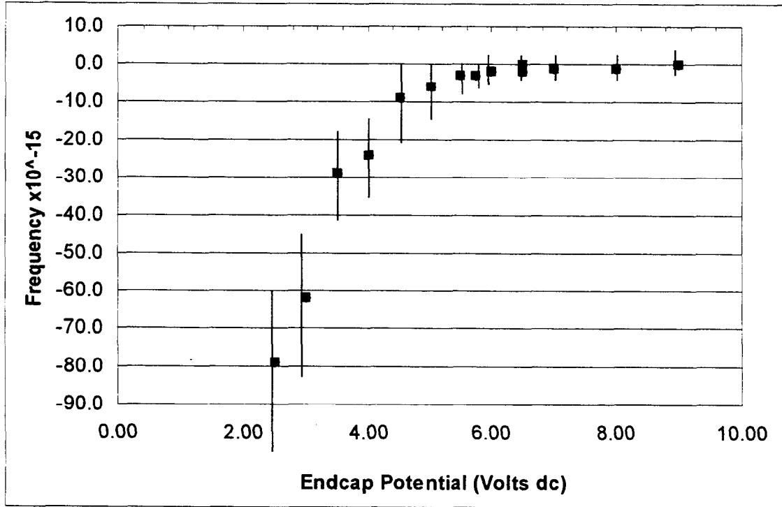
Figure 3: Second-Order Doppler frequency pulling as a function of ion number. The ion number is varied by changes in the endcap potential. This shift is twenty times less than observed with a similar number of ions in the traditional quadrupole linear ion trap.
