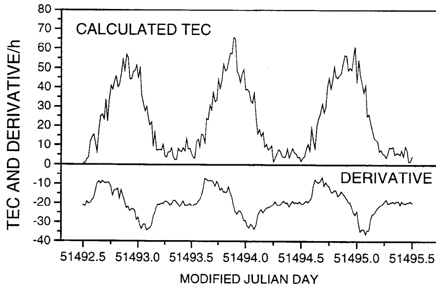
Figure 3. Values of TEC_v and the derivative TEC_v' calculated from 3 days of single-frequency measurements. The values of TEC_v' are scaled in TEC units per hour, and have been displaced -20 units for clarity.
