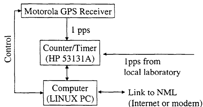
Figure 6: Schematic diagram of the NML GPSCV time-transfer system based on the Motorola VP Oncore GPS engine.
