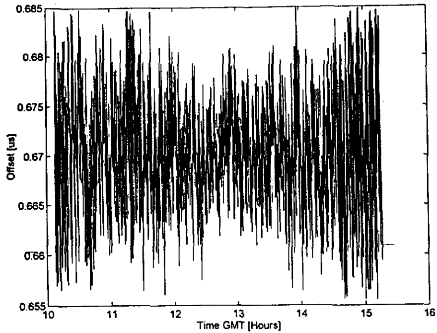
Figure 3: UTC(LDS) - UTC(NPL2) → PRN 4 on 4 Nov '94 mean value = 670.3 ns; 1-\sigma = 4.4 ns
