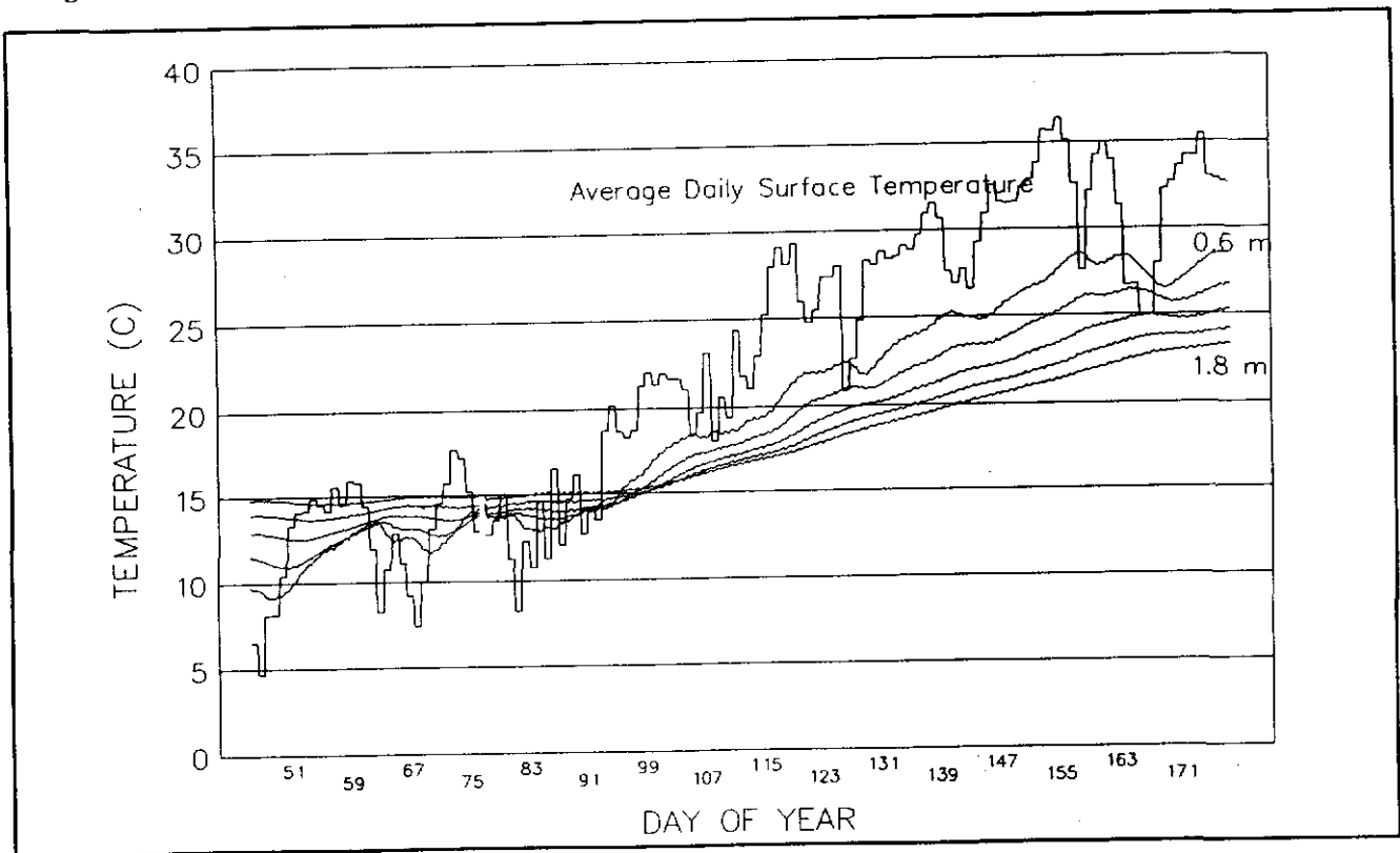
Figure 3. GROUND TEMPERATURE MEASURED AT GOLDSTONE TRACKING STATION
