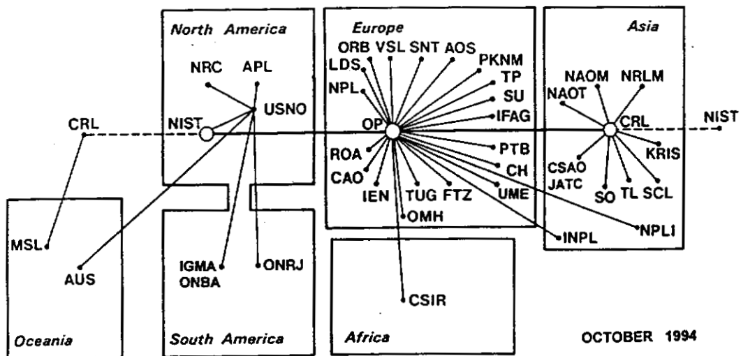
Figure 2. Organization of the international GPS time link network used for TAI computation (October 1994). Acronyms can be found in Table 3 of the Annual Report of the BIPM Time Section, Volume 6, 1994 .
