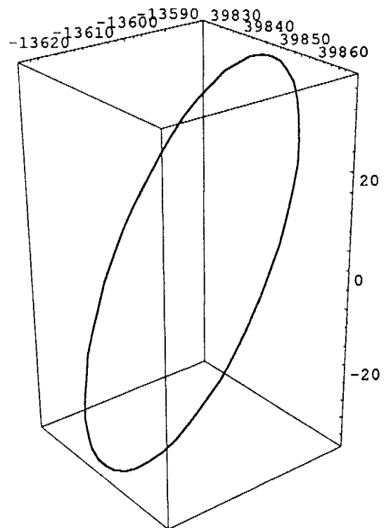
Figure 3 : Example of typical 24-hour residual orbit in a rotating reference frame (graduations in km).
