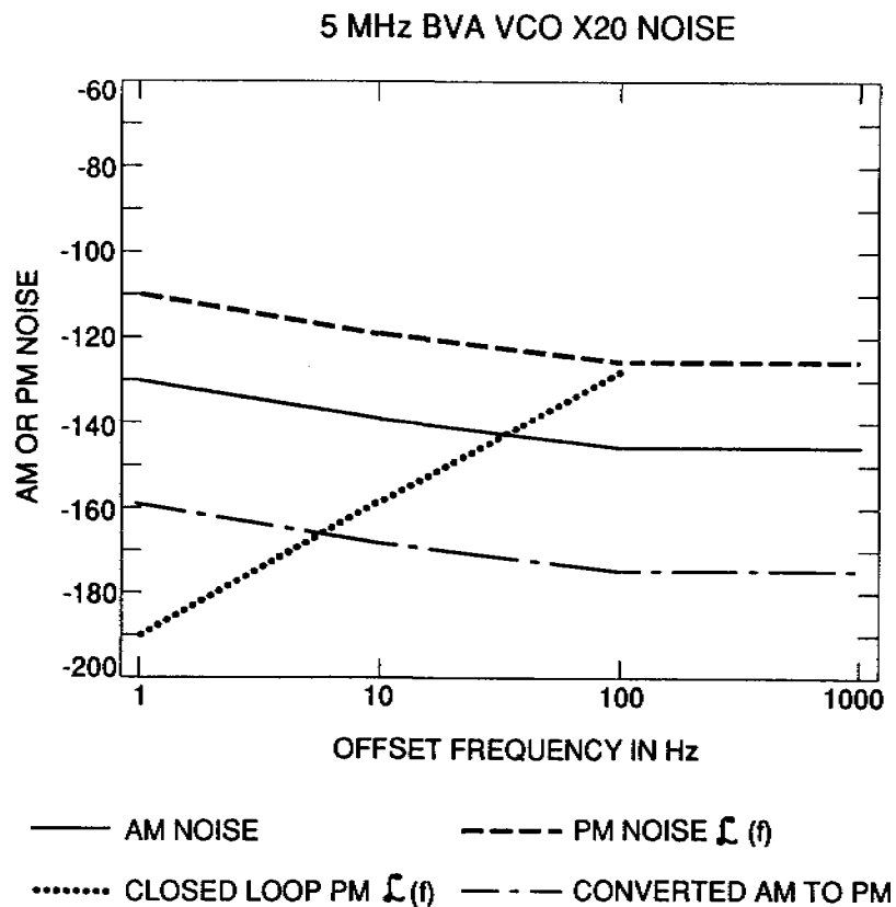
FIGURE 4b AM AND PM NOISE 5 MHz BVA VCO/x20 MULT.
