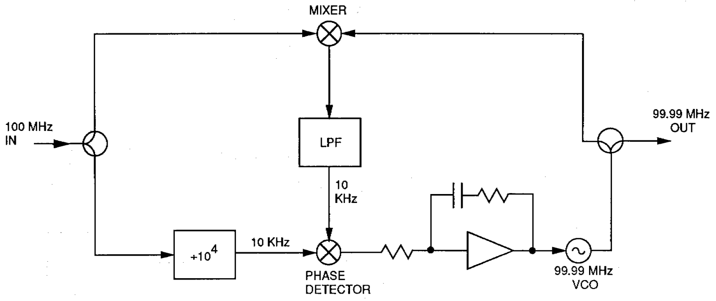
FIGURE 2 OFFSET GENERATOR BLOCK DIAGRAM
