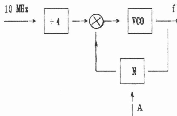
Fig. 6. 20.405 \pm f_m MHz Switched Synthesizer
