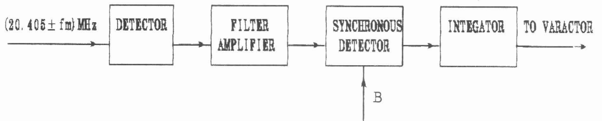
Fig. 8. Lock-in Amplifier
