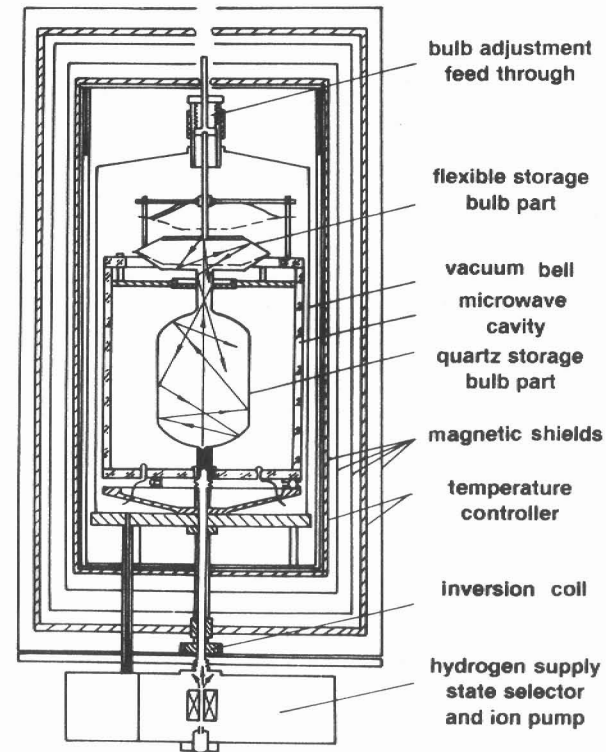
Fig.11. The hydrogen maser with flexible storage bulb.
