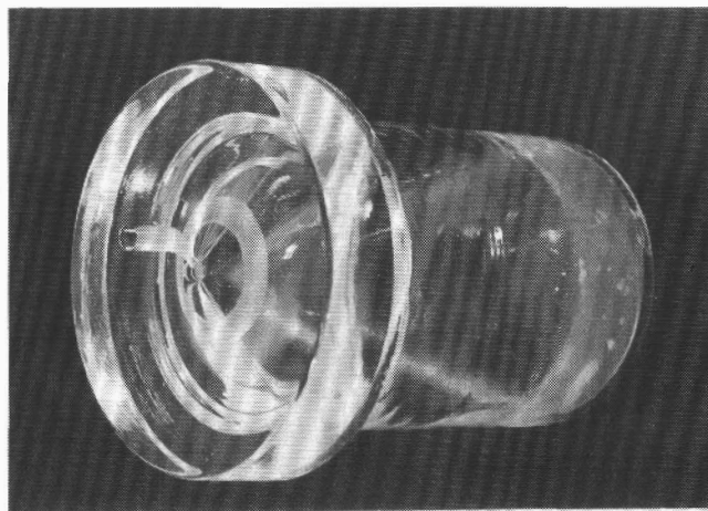
Fig.6. Quartz discharge bulb of hydrogen masers CH1-75, CH1-76.
