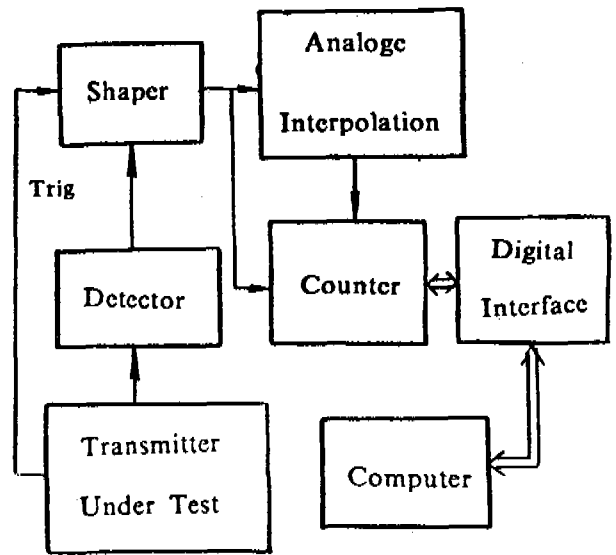
Figure 7. Time Interval Measurement Block Diagram
