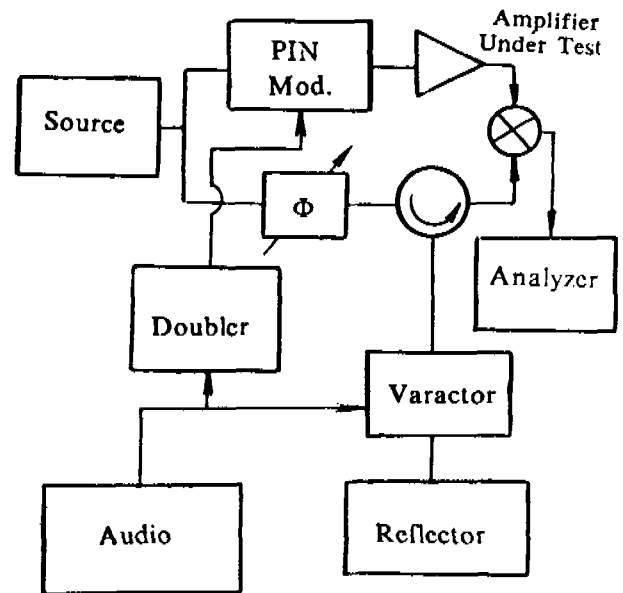
Figure 9. PM Calibration Block Diagram
