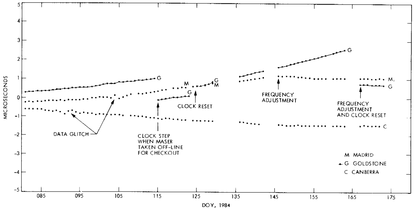
Figure 8. Time Offset, DFT System versus UTC (NBS), Showing All Three Stations
