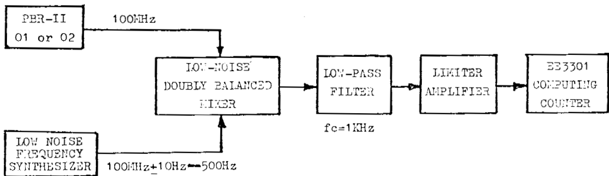
Fig.9. Experimental setup used in measurement of PBR-II frequency stability for averaging time \tau = 2^{ms} - 100^{ms} .
