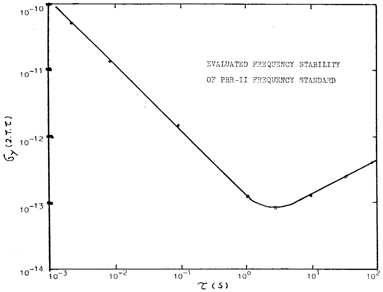
Fig.6. Evaluated time-domain frequency stability of PBR-II
