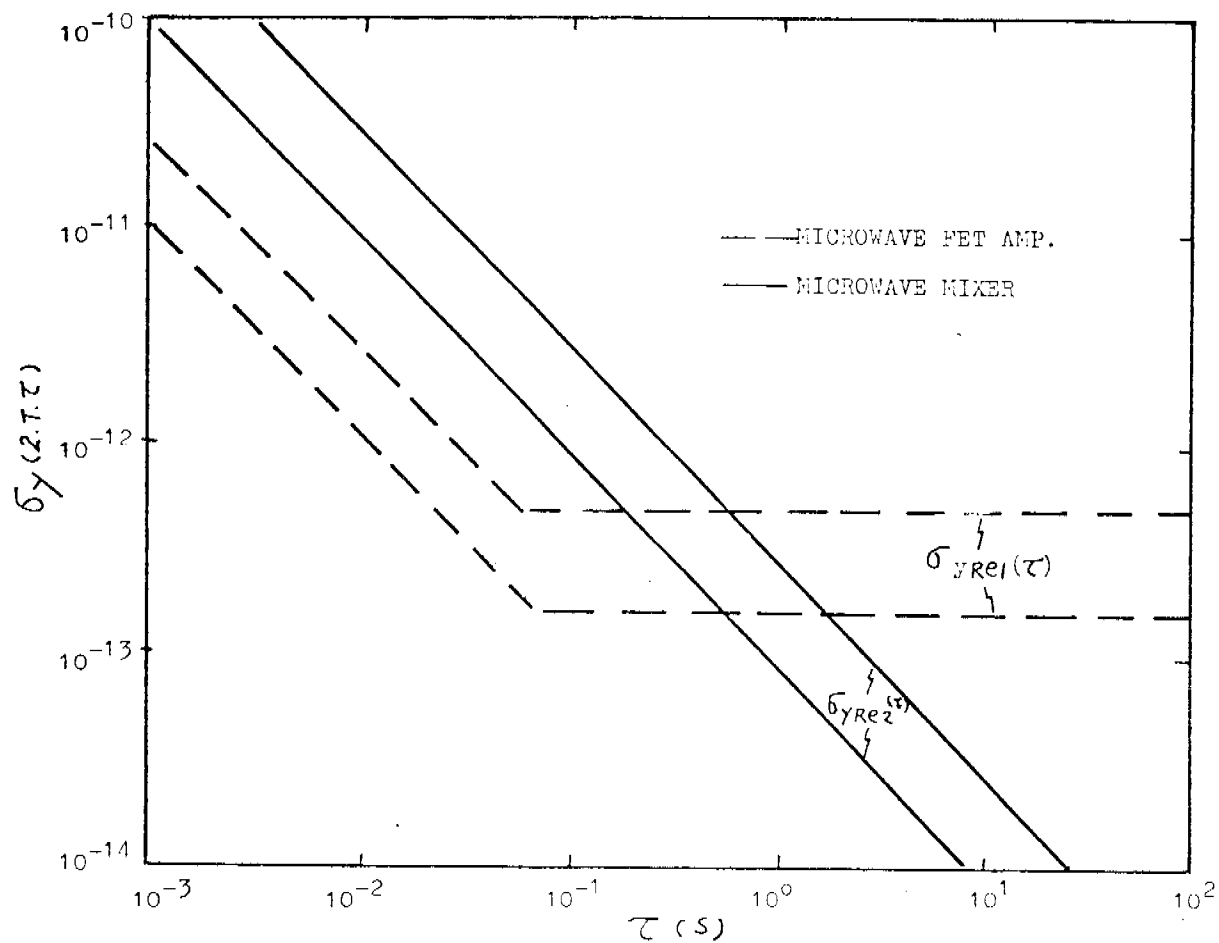
Fig. 5.b Time-domain frequency stability of two low-noise receivers.
