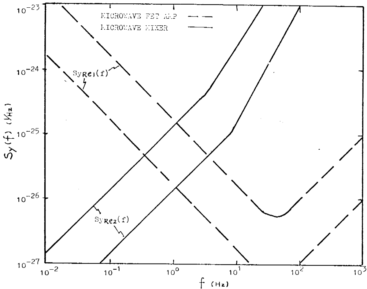
Fig.5,a Frequency-domain frequency stability of two low-noise receives.
