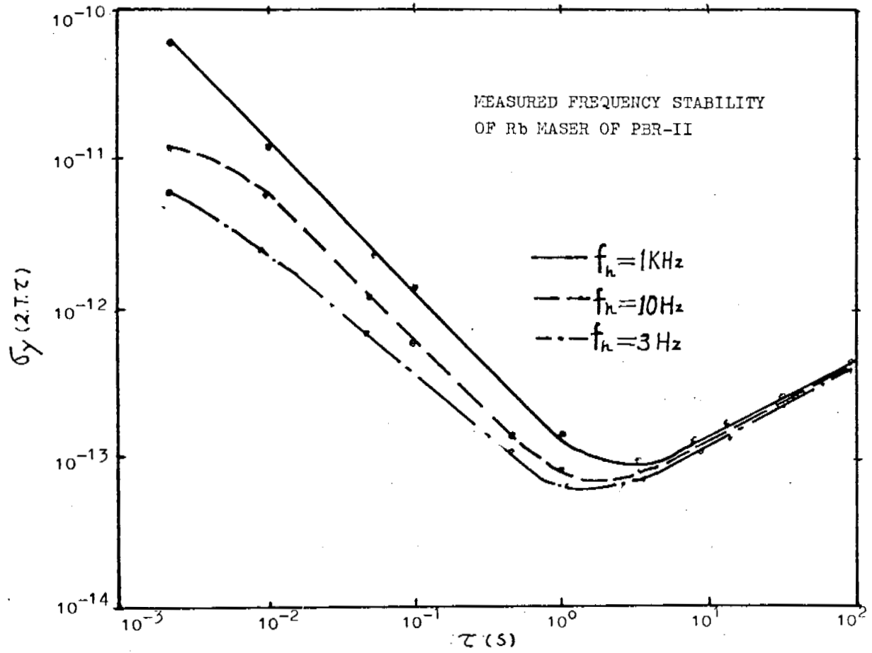
Fig.15. Time-domain frequency stability of Rb maser.
