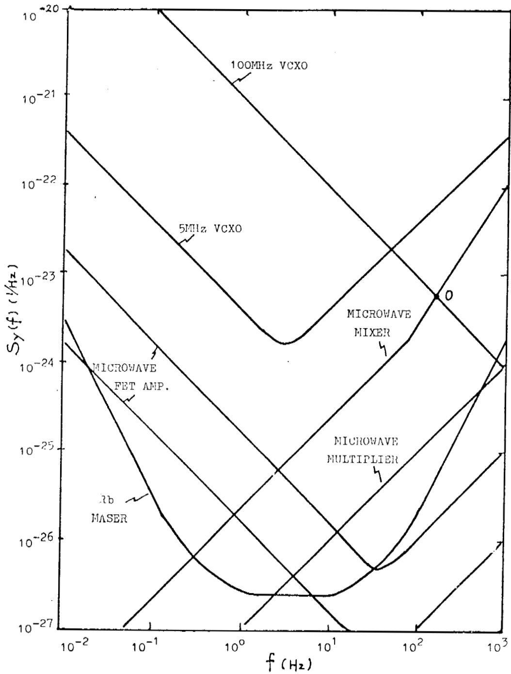
Fig.4. Frequency-domain stability of main components
