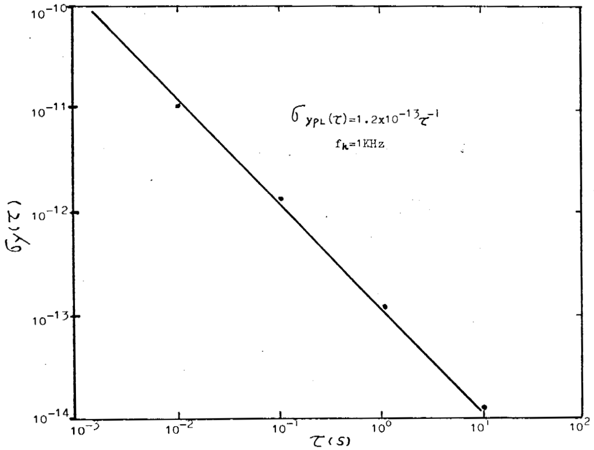
Fig.13. Phase-locked receiver noise contributions measured in the time-domain for f_k=1\text{KHz} .
