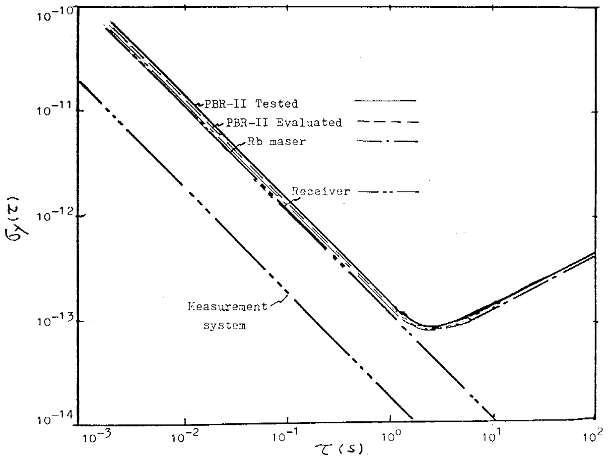
Fig.16. Time-domain frequency stability
