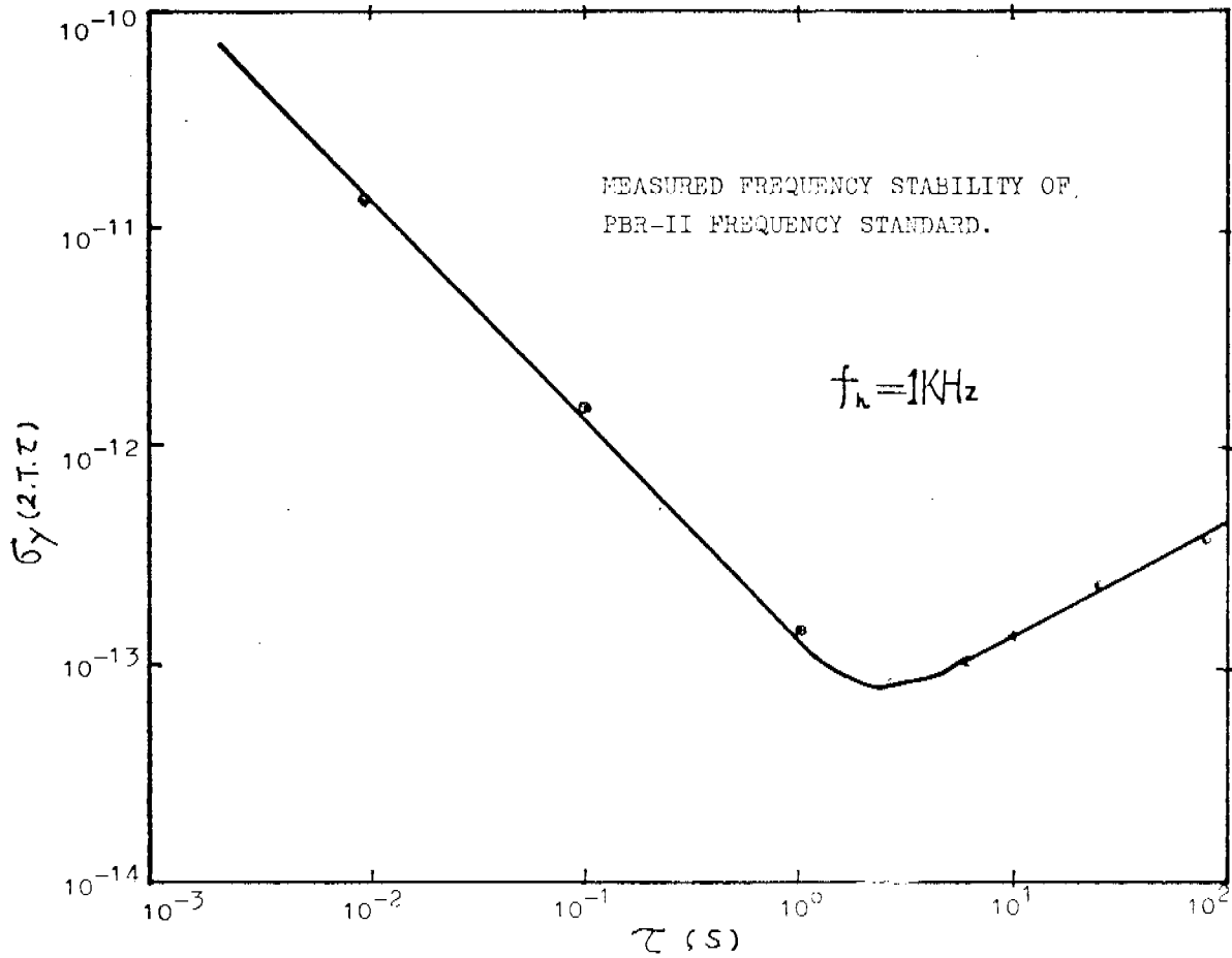
Fig.10. Actual tested time-domain frequency stability of PBR-II
