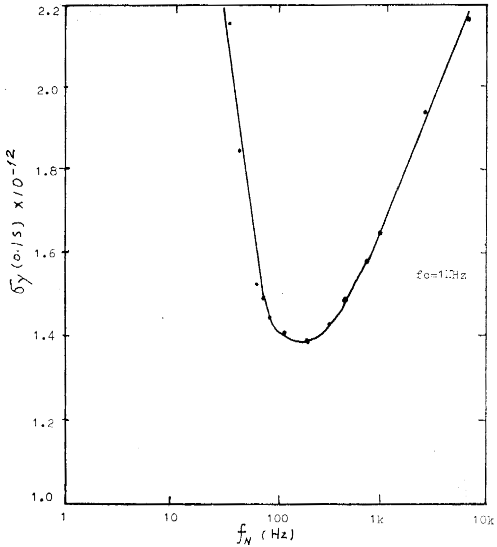
Fig.7. Evaluated value of the time-domain frequency stability \sigma_y(0.1s) versus loop nature frequency f_N for \tau = 0.1^s , f_c = 1\text{kHz} .
