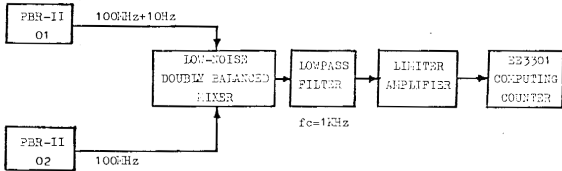
Fig.8. Experimental setup used in measurement of PBR-II frequency stability for averaging time \tau = 100^{ms} - 100^s .
