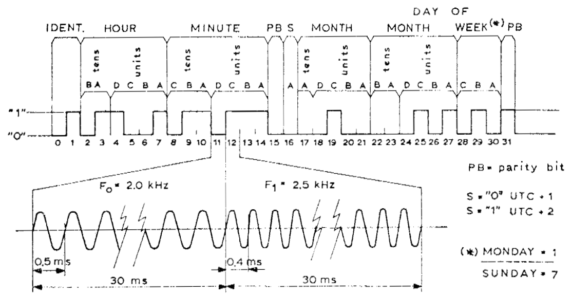
Fig.3 - Coded time signal broadcasted by the National Radio Company
