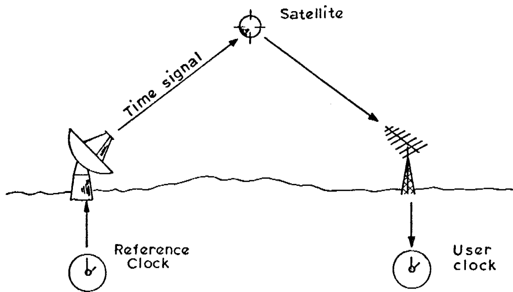
Fig.1 - One-way time dissemination via satellite
