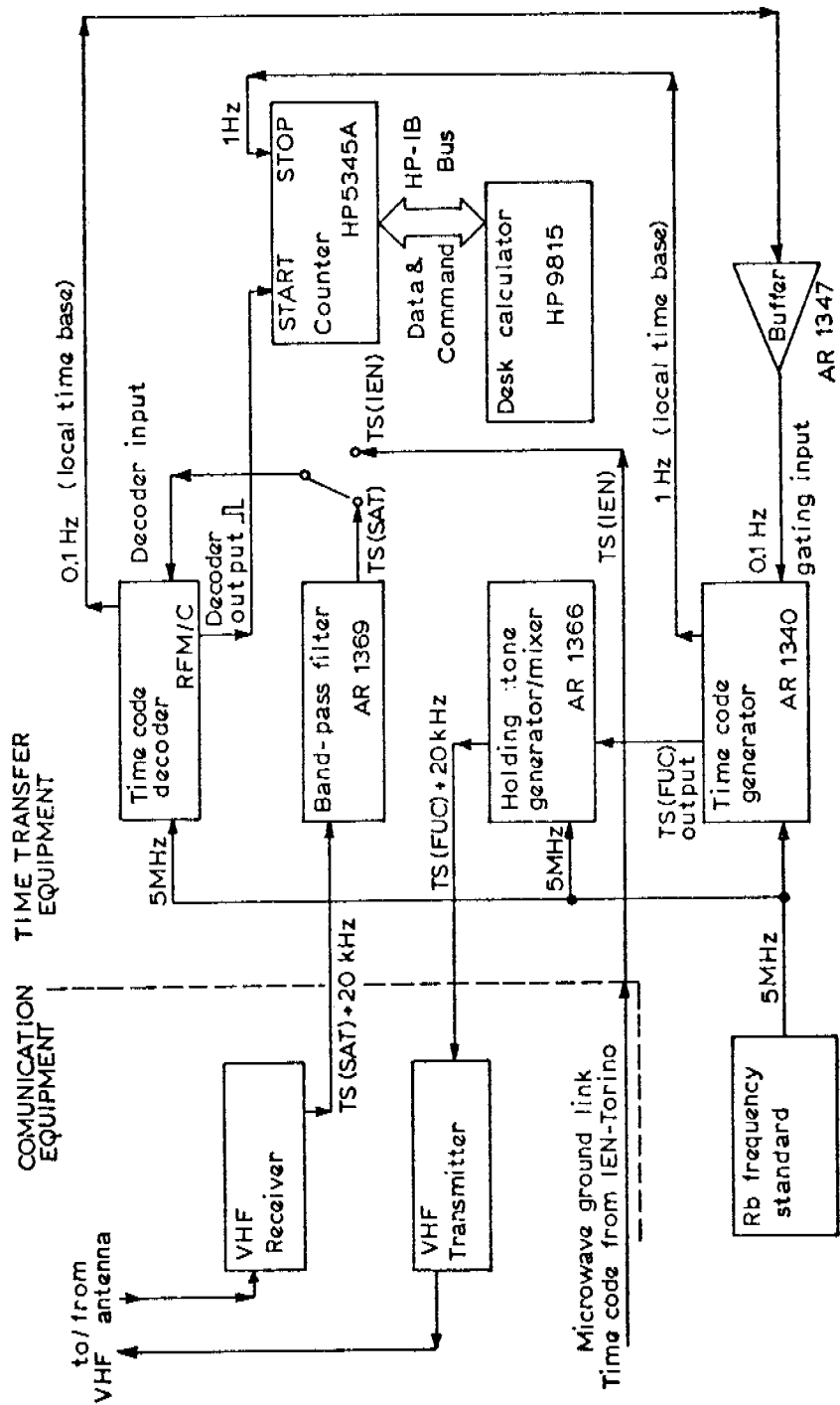
Fig.4 - Experimental set-up (Fucino ground station) TS = Time signal
