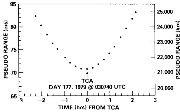
Figure 2—Typical NAVSTAR pseudo-range signature, plotted every 15 minutes
