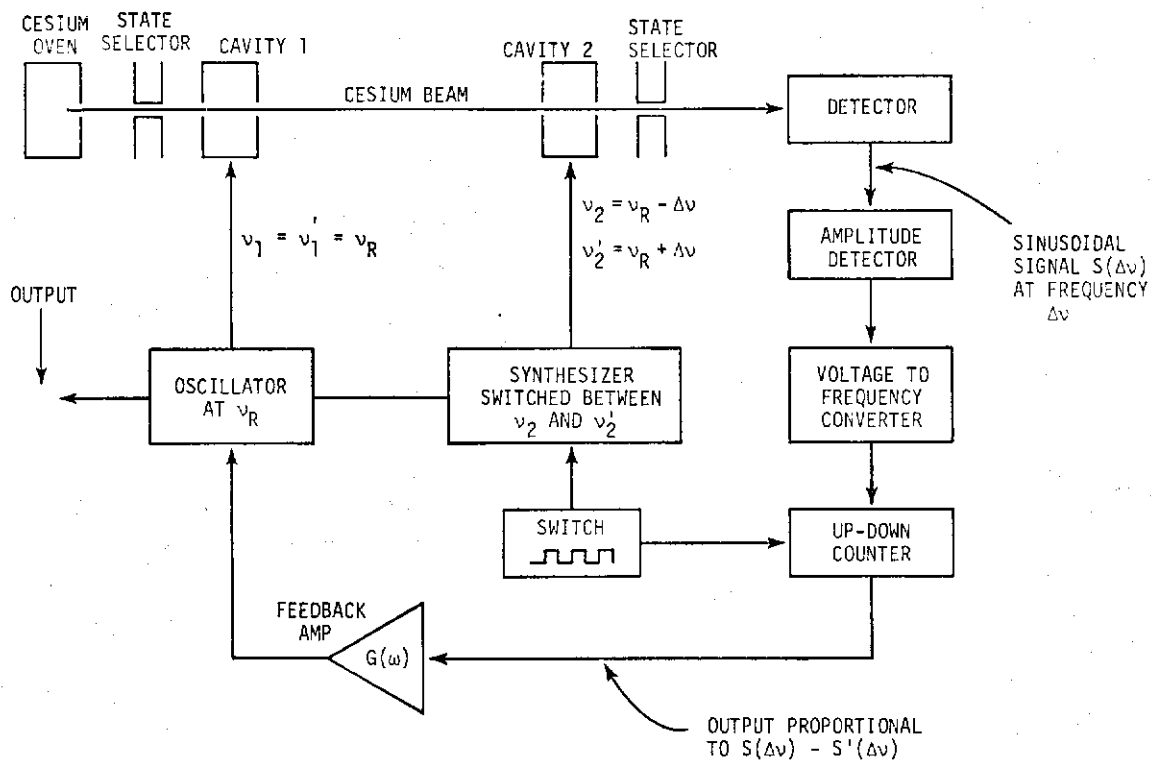
Figure 5. Simplified Diagram of One Possible 2 Cavity-2 Frequency Configuration. [11]
