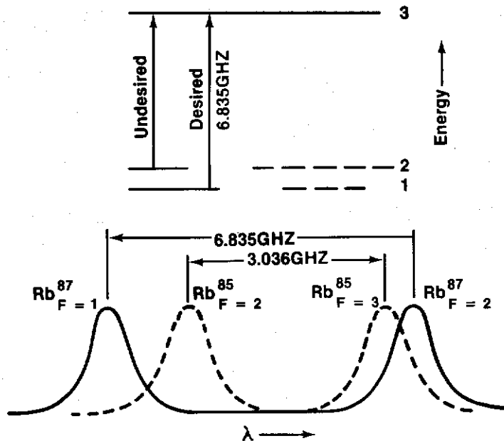
Figure 2. Levels of Interest for Optical Pumping of Rubidium
