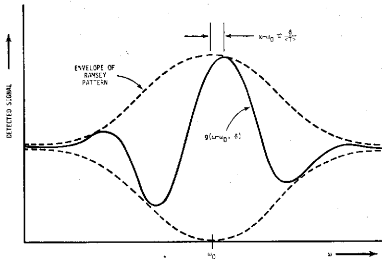
Figure 6. Ramsey Pattern for a Phase Shift Between the Two Cavity Ends. Dotted Line Shows the Ramsey Envelope
