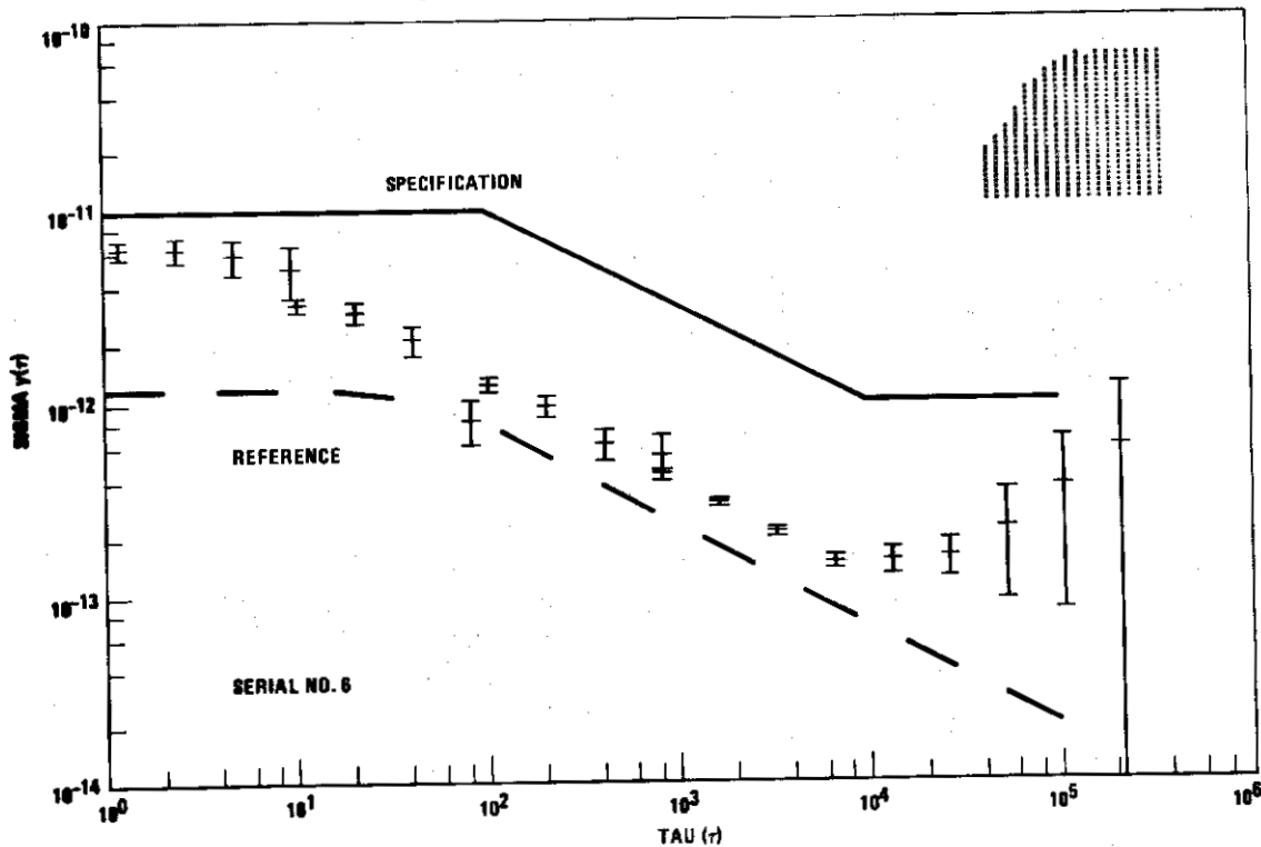
Fig. 8—Computer Printout of Allan Variance Plot
