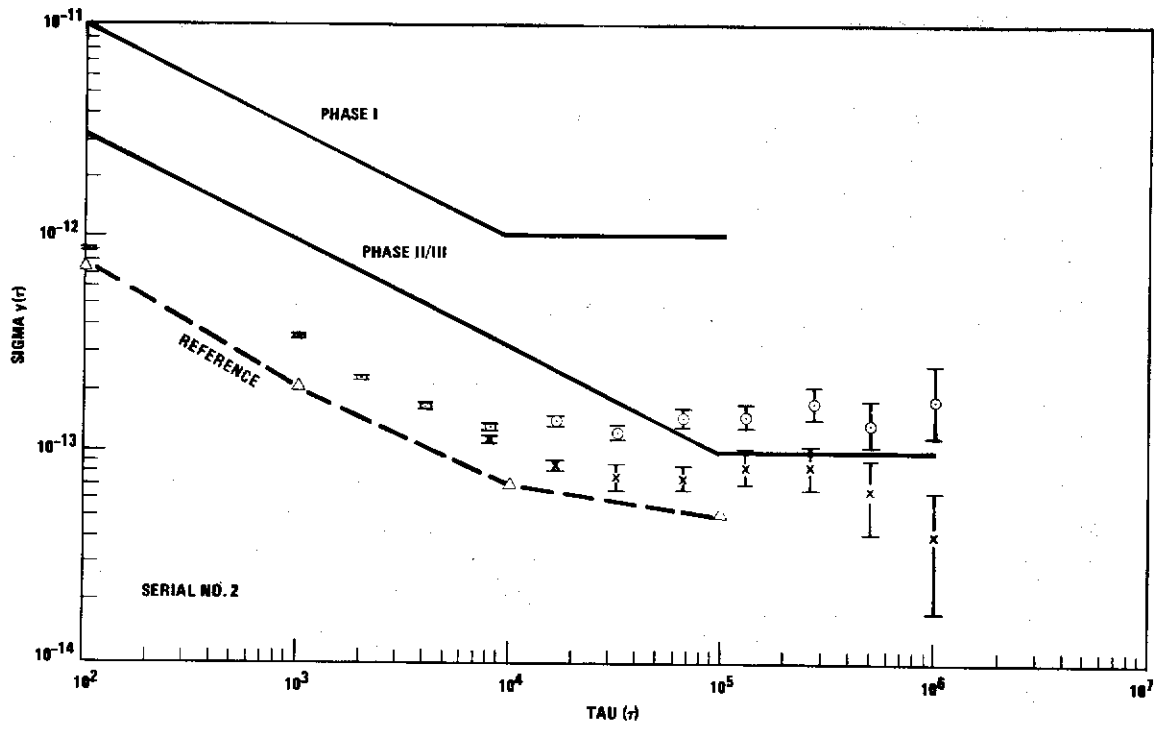
Fig. 16—Allan Variance Plot/Life Cycle Test
