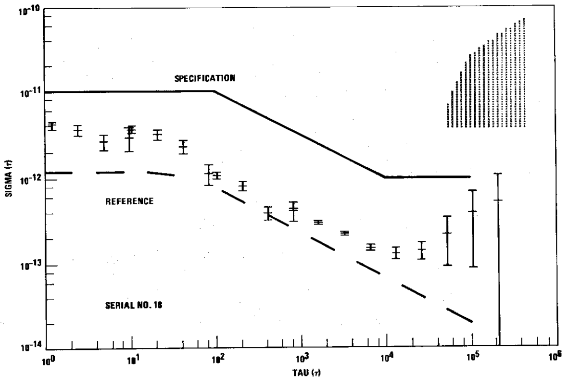
Fig. 11—Computer Printout of Variance Plot
