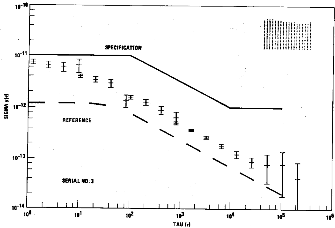
Fig. 9—Computer Printout of Allan Variance Plot
