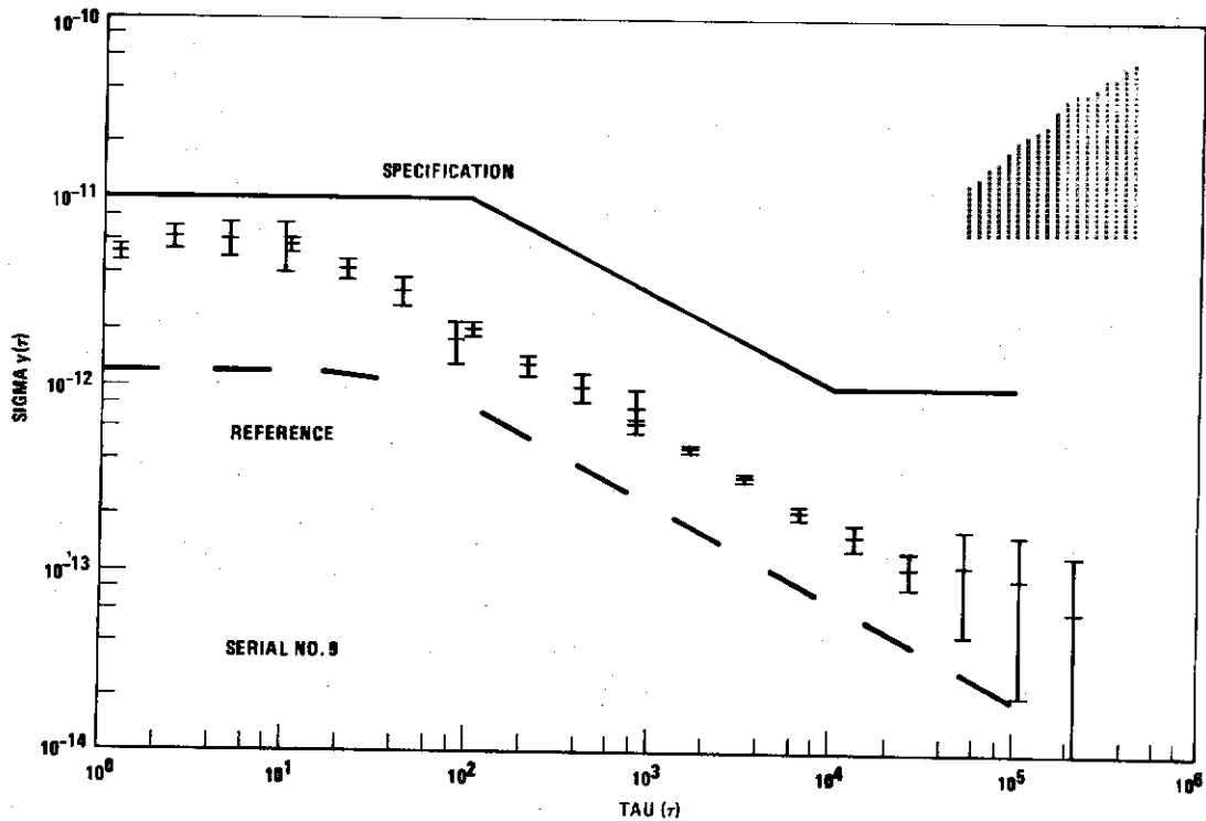
Fig. 10—Computer Printout of Allan Variance Plot
