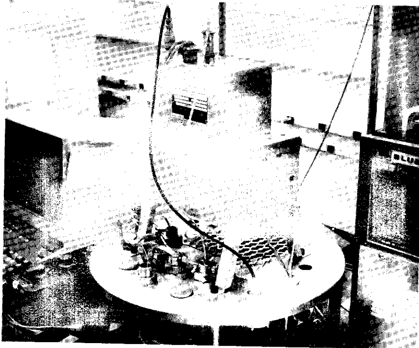
Fig. 5—Rubidium Frequency Standard
