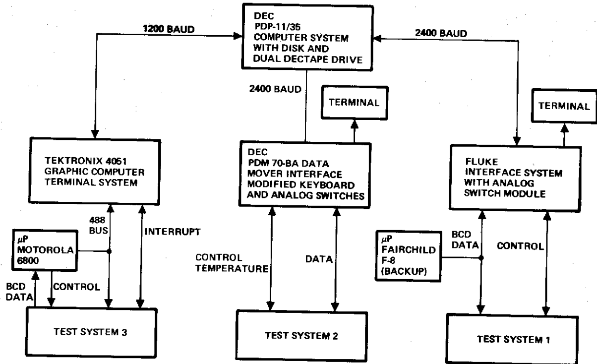
Fig. 1—Overall Automated Test Systems
