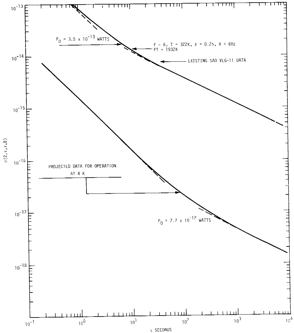
Fig. 5—Projected improvements in hydrogen-maser stability due to low-temperature operation.
