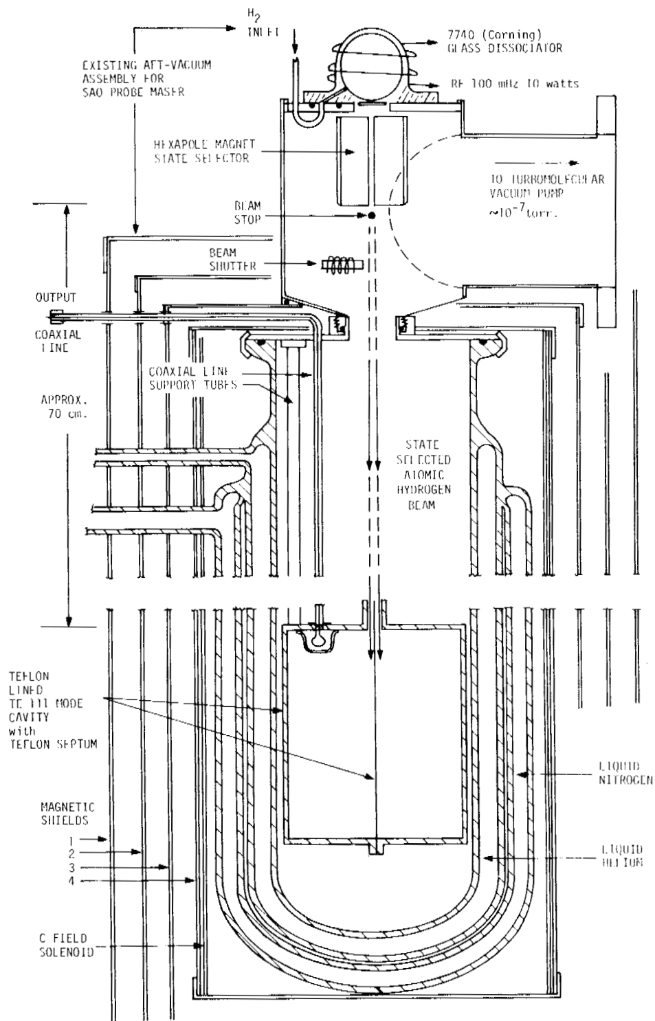
Fig. 7—Schematic view of low-temperature atomic hydrogen maser.
