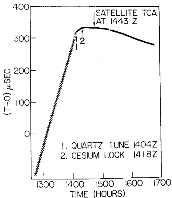
Fig. 19 - Cesium frequency standard lock up, 1977 day 190, 1418 UTC
