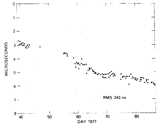
Fig. 29 - NTS-1 time transfer, NASA Cape Kennedy Station
