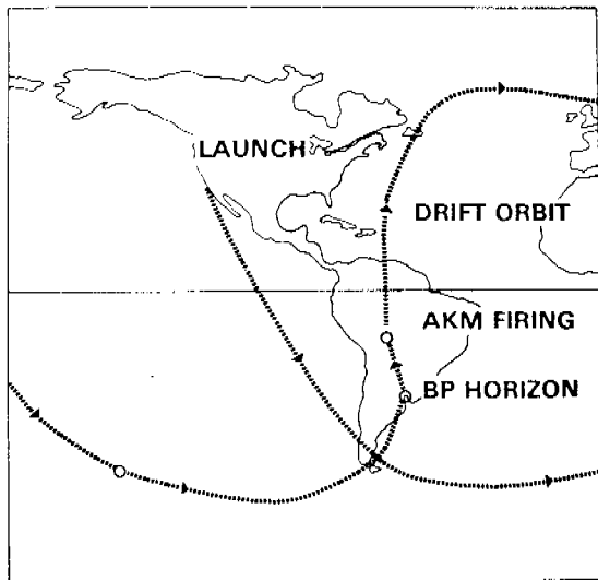
Fig. 4 - NTS-2 transfer orbit
