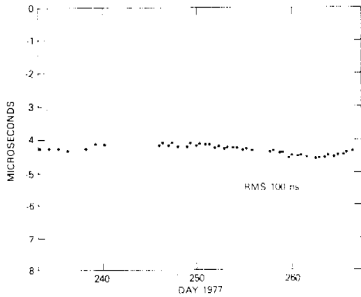
Fig. 30 - NTS-2 time transfer, NASA Cape Kennedy station
