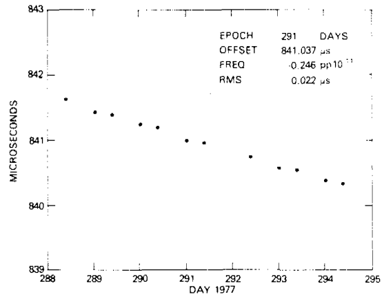
Fig. 25 - Frequency, NTS-CBD after C-field adjustment, 1977 day 287
