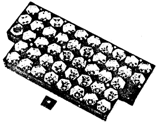
Fig. 35 - NTS-2 laser retroreflector
