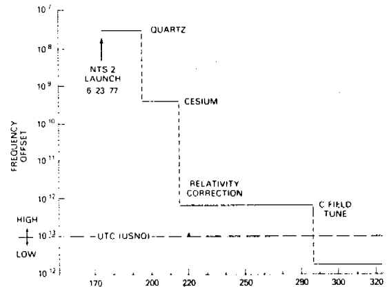
Fig. 27 - Frequency offset summary
