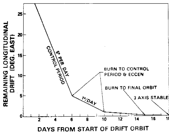
Fig. 8 - Pre-launch NTS-2 drift orbit profile
