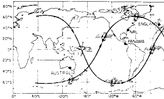
Fig. 10 - NAVSTAR GPS Phase I orbit traces
