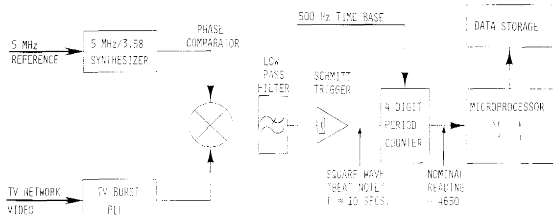
Fig. 2-Block diagram, 3,58 MHz fractional frequency measurements
