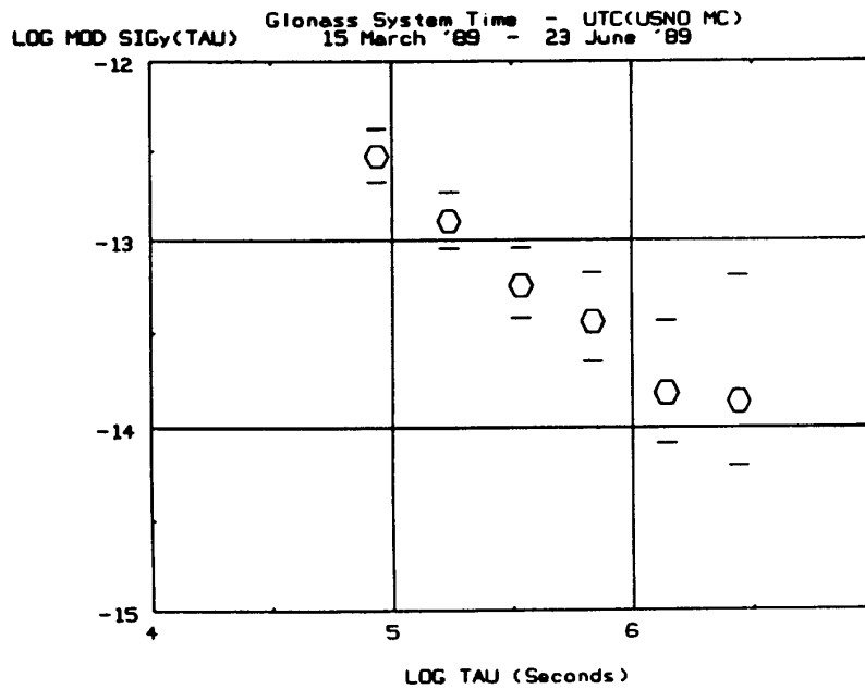
Figure 9. A plot of the fractional frequency stability, \text{mod}\sigma_y(\tau) , of the smoothest part of the data plotted in Figure 8. The \tau^{-1} behavior is modeled by flicker noise PM. This is not characteristic of the clocks involved.
