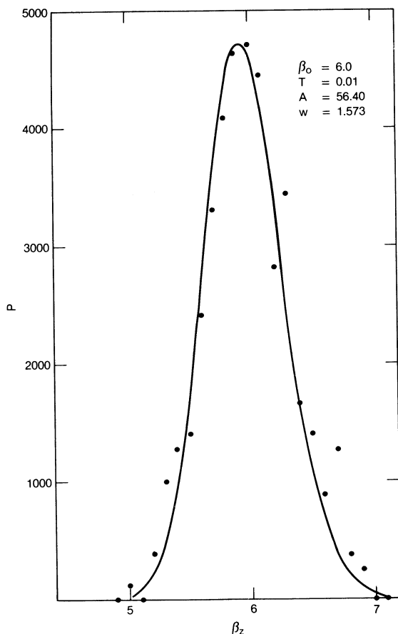
FIG. 5. P_1 fit to computer simulation data plotted as a function of \beta_z with \beta_p=0 and \beta_\phi arbitrary.
