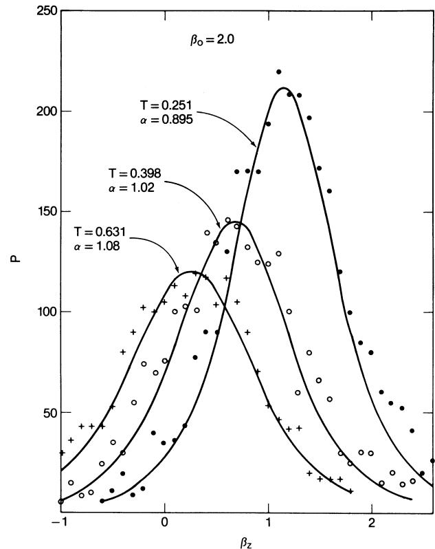
FIG. 15. Fit to computer simulation data for \beta_0=2 using Eq. (3.7). Results are plotted as a function of \beta_z for \beta_\phi=0 and \beta_\phi arbitrary. Each curve is labeled by the normalized time variable T .
