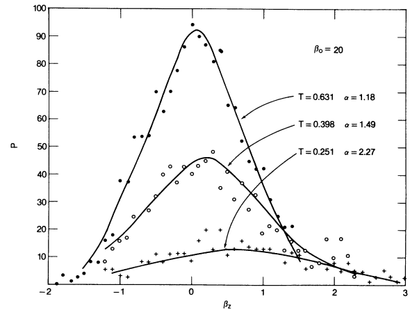
FIG. 14. Fit to computer simulation data for \beta_0=20 using Eq. (3.7). Results are plotted as a function of \beta_z for \beta_\phi=0 and \beta_\phi arbitrary. Each curve is labeled by the normalized time variable T .
