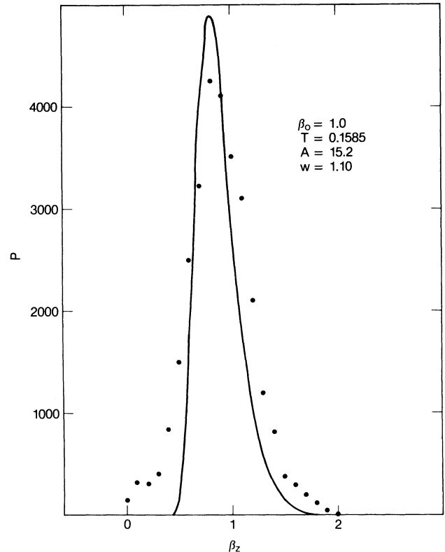
FIG. 10. P_1 fit to computer simulation data plotted as a function of \beta_z with \beta_\rho=0 and \beta_\phi arbitrary.
