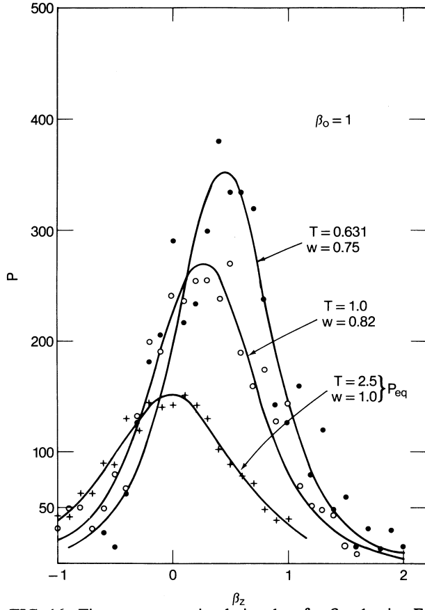
FIG. 16. Fit to computer simulation data for \beta_0 = 1 using Eq. (3.7). Results are plotted as a function of \beta_z for \beta_p = 0 and \beta_\phi arbitrary. Each curve is labeled by the normalized time variable T .
