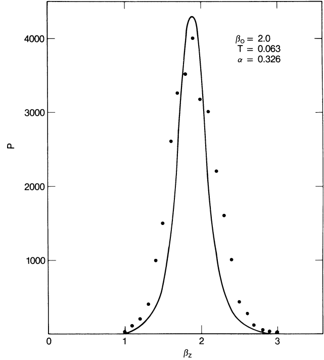
FIG. 17. Fit to computer simulation data using Eq. (3.7) plotted as a function of \beta_z for \beta_p = 0 and \beta_\phi arbitrary.
