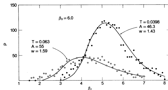
FIG. 6. P_1 fit to computer simulation data plotted as a function of \beta_z with \beta_p=0 and \beta_\phi arbitrary.
