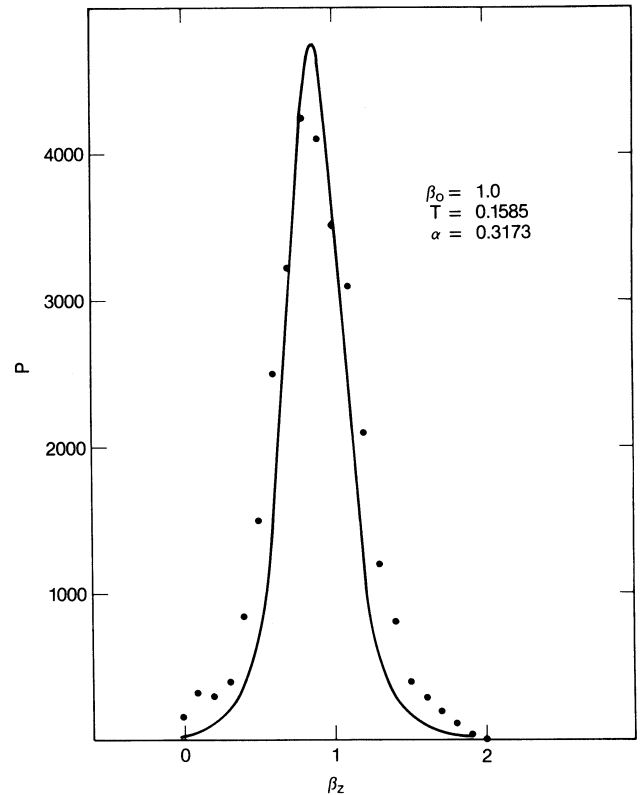
FIG. 18. Fit to computer simulation data using Eq. (3.7) plotted as a function of \beta_z for \beta_p = 0 and \beta_\phi arbitrary.
