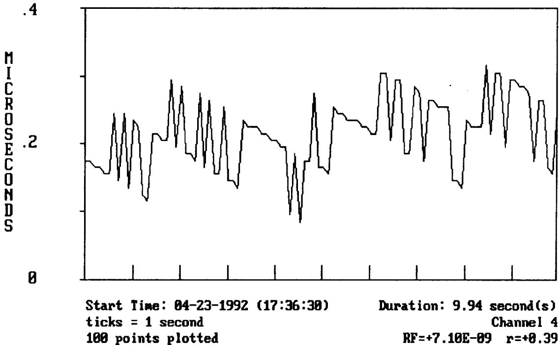
Figure 4. LORAN-C path variations over a 10-second period.
