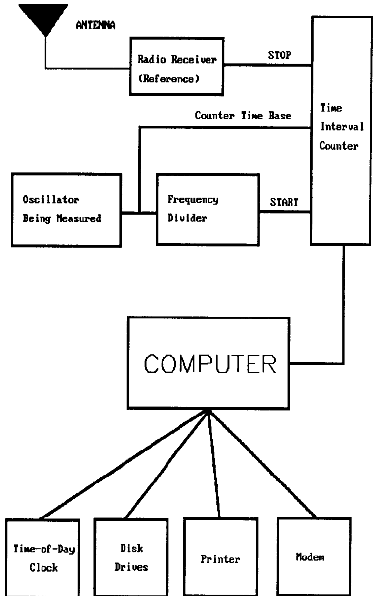
Figure 3. Block Diagram of the NIST Frequency Measurement System.
