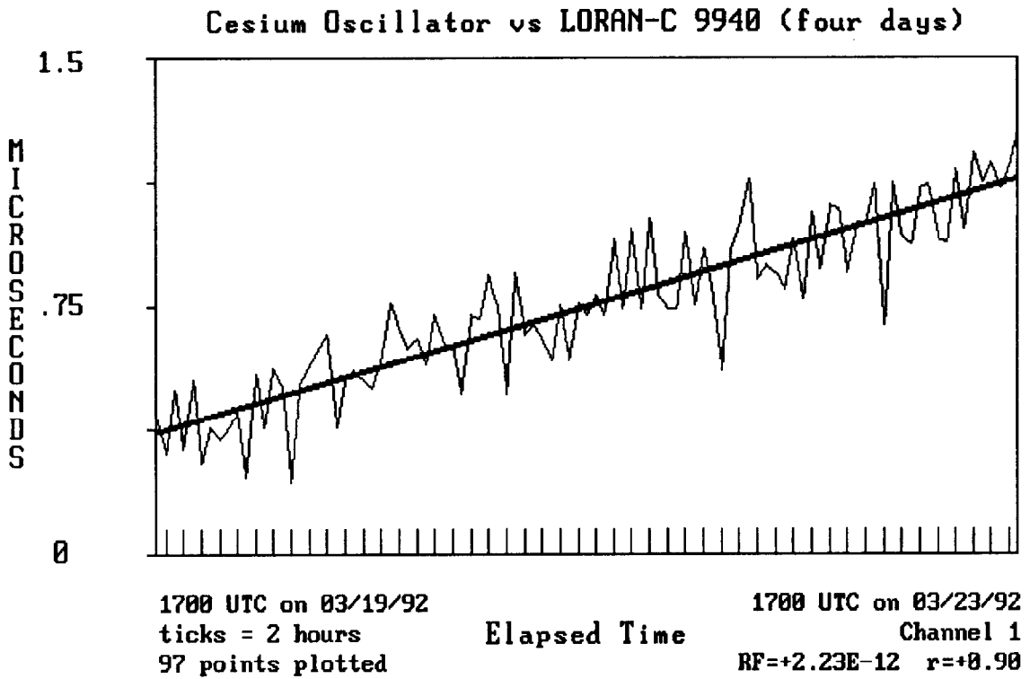
Figure 10. A 96-Hour comparison of a Cesium Oscillator to LORAN-C.
