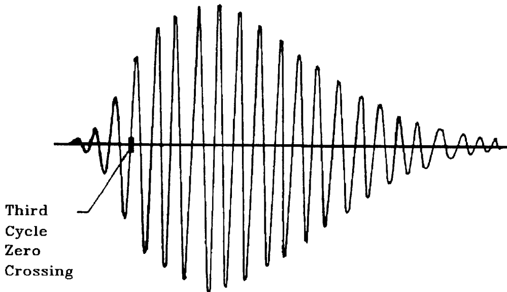
Figure 2. A LORAN-C Pulse with the Third Cycle Identified.
