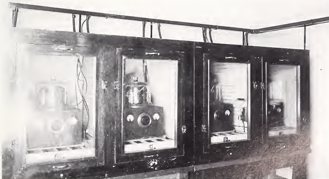
In 1929 these four 100-kHz quartz oscillators, with auxiliary circuitry and temperature-control equipment, were installed in the Radio Building, to become the National Primary Standard of Radio Frequency.
