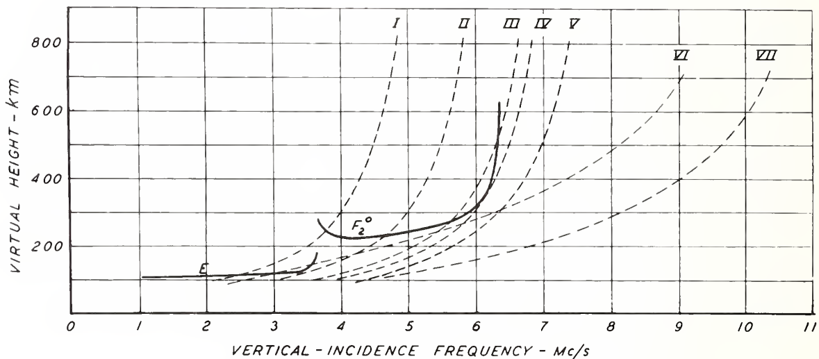
Earliest published (July 1937) transmission curves by NBS for determination of frequency for selected distances of transmission (assuming flat Earth and flat ionosphere). In a generalized form, this whole procedure by Newbern Smith shows the various relationships. The solid curve is a typical normal-incidence observation of virtual height vs. frequency, showing the E and F_2 layers of the ionosphere. The dotted curves depict conditions of transmission for various frequencies and several distances. For example, curve IV depicts maximum possible frequency for a given distance. Adoption of this method became valuable for predicting median values of maximum usable frequency for propagation over any path at any time of day for several months ahead, and provided for world charts during World War II for predictions.
