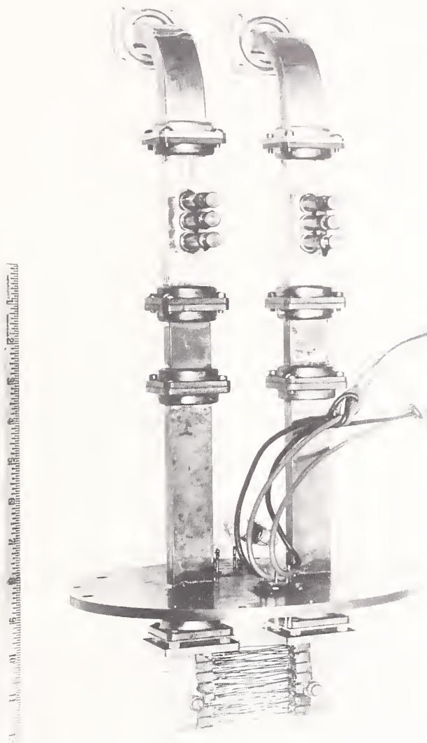
Waveguide section of the first of a series of microwave microcalorimeters (Joule twin type) developed by NBS, this one by Macpherson and Kerns, beginning in 1948. Earliest model used polyiron as the absorbing load at about 1 milliwatt of RF power; replaced in later models with a bolometer unit. A dummy load served as the temperature reference for the multi-junction thermopile (lowest portion of photograph). Tuning stubs (upper portion) provided impedance matching of X-band assembly at 9315 MHz. Entire unit was temperature controlled in a 45-gallon oil bath.
