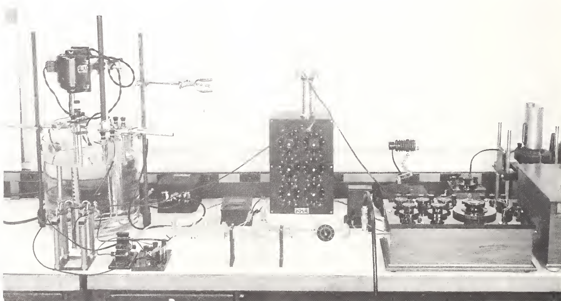
Microwave power measurements in 1946, using a thermistor mounted in coaxial power mount. Control of ambient temperatures of mount was by a makeshift 10-gallon constant temperature water bath with a stirring device. Sophisticated types of oil and water baths were to come later. Microwave power was in terms of equivalent DC power, using standard resistors, a standard cell, and potentiometer for measurement.
