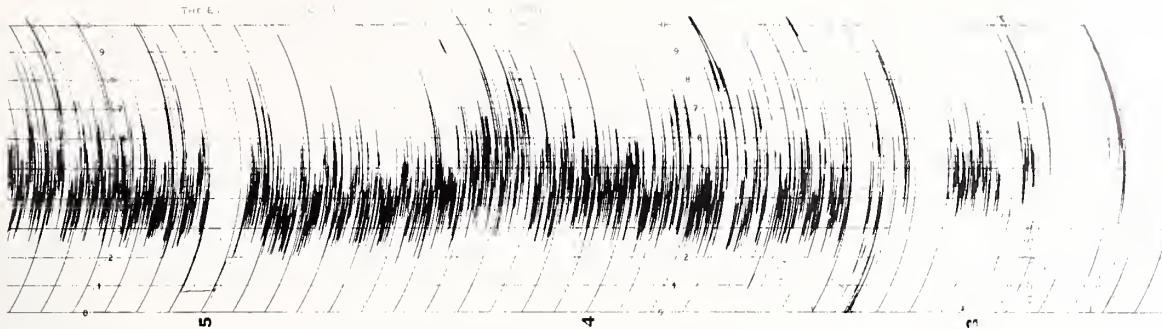
Chart tracing of VHF signals observed for the first time by ionospheric forward scatter. On the evening of January 23, 1951, signals were transmitted from Cedar Rapids, Iowa and received at the NBS Sterling field station over a 1243-km path. After preliminary adjustment of the equipment, a signal trace was received at 2250 (10:50 p.m.) and, then upon further adjustment, signals were received continuously from 2255 until mid morning of the following day (January 24). The reading speed was at 1 ft per hour, the tape moving from right to left. The initial trace is approximately 3 1/2 divisions to the right of "3," then follows the more continuous tracing beginning about 1 division to the right of "3." At "5" and continuing for 1 division is an indication of the noise level, which was substantially less than the signal level. The signal tracings are on an arbitrary scale. However, subsequent observations showed signal levels ranging from 10 to 25 decibels above 1 microvolt.
