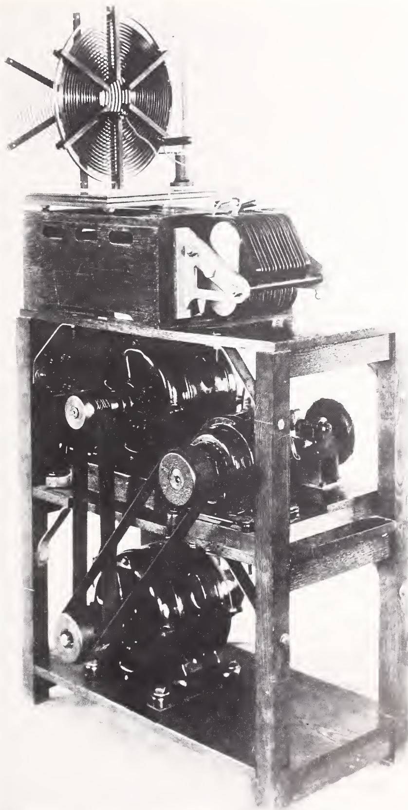
One-half-kilowatt spark transmitter designed by Radio Section for automatic and continuous coding of signals. This and other types of transmitters were used at lighthouses in the Lower New York Bay area for radio "fog signaling" experiments by the Radio Section and Bureau of Lighthouses, beginning in 1917 and extending to the mid-1920's.
