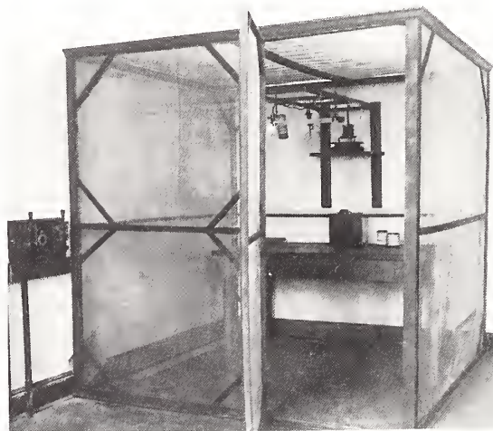
An early shielded room or "cage" developed by the Radio Section. The first attempt at shielding was in 1917 with considerable success in minimizing the strong signals of NAA, the powerful Navy station across the Potomac in Arlington, Va.
