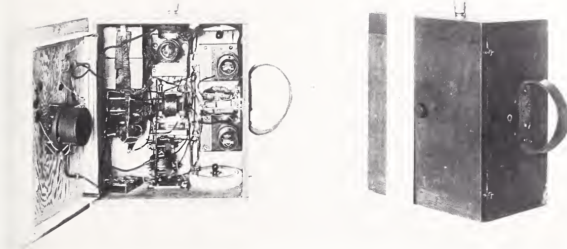
The "Portaphone," a portable radio receiver constructed by the Radio Section in 1921. Included within the wood case (12×12×6 in) was a loop antenna with tuning capacitor, electron-tube detector, two-stage amplifier, and dry batteries. A loudspeaker driver unit fitted with a small "morning glory" horn provided sufficient volume to entertain the passerby with music from local broadcasting stations. A later model completely enclosed a wood horn.
