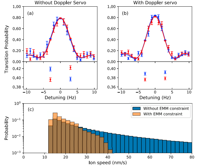
FIG. 3. First-order Doppler shift characterization. (a) Clock transition line shapes for the two opposing probe directions (red and blue points) measured during clock operation without a first-order Doppler servo. Solid lines show fits to a Rabi line shape. The enlarged view shows that the transition probabilities at the probe frequencies used for the frequency lock are not balanced for each direction individually, indicating a non-zero first-order Doppler shift. (b) Similar data taken while running the first-order Doppler servo, with balanced transition probabilities at the lock points. (c) Distribution of possible ion speeds based on the measured first-order Doppler shift with and without an additional velocity constraint from EMM measurements.
