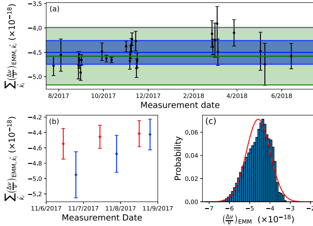
FIG. 2. Excess micromotion shift evaluation. (a) The sum of the EMM frequency shifts (black points) measured along three nearly orthogonal probe directions from August 2017 to June 2018, with the average and standard deviation (blue line and band). (b) Sample of EMM measurements on three consecutive days. Red points are data taken immediately after initial EMM compensation and blue points are data taken after \approx 12 hours of clock operation with interleaved micromotion compensation servos. (c) Histogram of possible total EMM shifts consistent with the measurements generated by a Monte Carlo analysis accounting for the non-orthogonality of the probe directions and assuming the worst-case scenario of either 0 or \pi phase of ion motion along these directions. The total EMM shift of \Delta\nu/\nu = -(45.8 \pm 5.9) \times 10^{-19} is given by the mean and standard deviation of the calculated distribution and shown in (a) (green line and band). For reference, the red line shown in (c) is a normal (Gaussian) distribution with the same mean and standard deviation.
