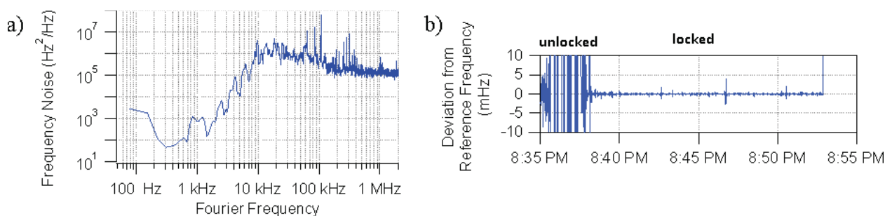
Figure 3: Results of the O-band tunable laser locked to the THz comb. (a) In-loop PSD of locked frequency noise, and (b) 1 second gate in-loop counter measurement for locking greater than 15 minutes.
