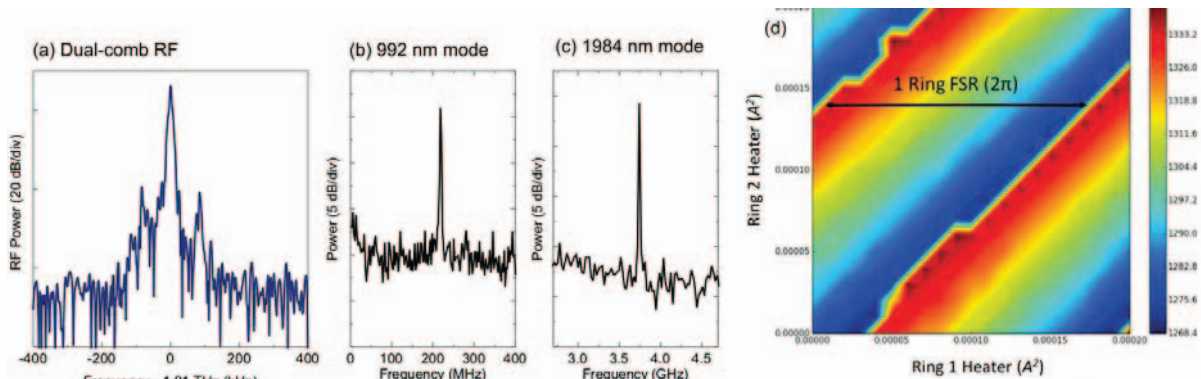
Figure 2: RF outputs of the dual Kerr comb indicating low-noise operation. (a) Repetition rate beat between the pump THz and silica comb, (b) 992 nm heterodyne beat with the second harmonic generation of the ECDL, and (c) 1984 nm heterodyne with the ECDL. (d) Tuning map of the O-band tunable laser for this demonstration, showing mode hop free tuning using the two ring resonators.
