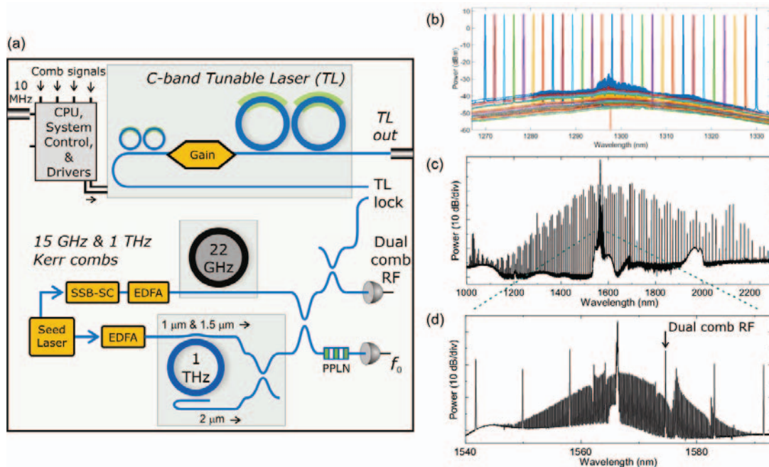
Figure 1: Heterogeneous photonics system for optical frequency synthesis. (a) System components include a Vernier ring tunable laser with III/V-Si heterogeneous integration, and a dual microresonator Kerr comb based on a 22 GHz silica device and a 1 THz silicon-nitride device operating in the low noise soliton regime. (b) Tunable laser tuning spectra for this demonstration. (c) Octave-bandwidth dual Kerr comb with dual dispersive waves for f-2f self-referencing and dense mode spacing near the 1550 nm pump. (d) Zoom of (c) showing the dense 22 GHz silica comb.
