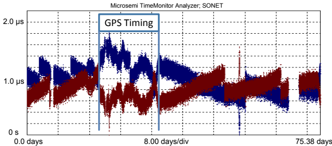
Fig. 3. Data as in Figure 2 with the minimum offset of each nulled to show the deviations. For most of this period the nodes were timed by Cs clocks, showing a slope of about 50\ \text{ns/d} with occasional resets of about 300\ \text{ns} . A
