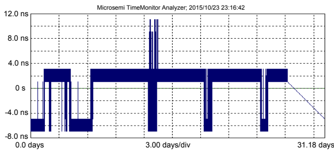
Fig. 9. PTP over OTN data after the differencing operation for time transfer shows no slope as the forward and reverse slopes cancel out.
