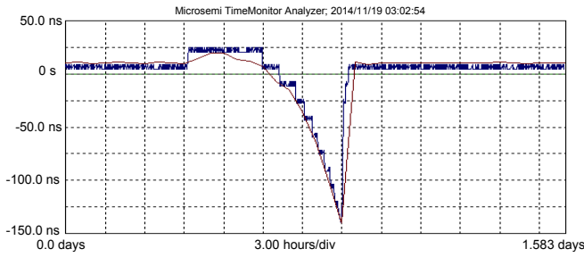
Fig. 12. During a period with a failure of timing equipment, the PTP remote measurement (red) matches the local measurement (blue). The 4 ns PTP precision and 16 ns granularity of steps are visible.
