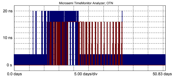
Fig. 5. PTP over OTN data with the minimum offset nulled shows a peak-to-peak variation of 20\ \text{ns} over 51\ \text{days} . Part of this is an apparent trend in the data, first up and then back. In the short term, the stability is 4\ \text{ns} , which is the resolution of the PTP measurement system we used.
