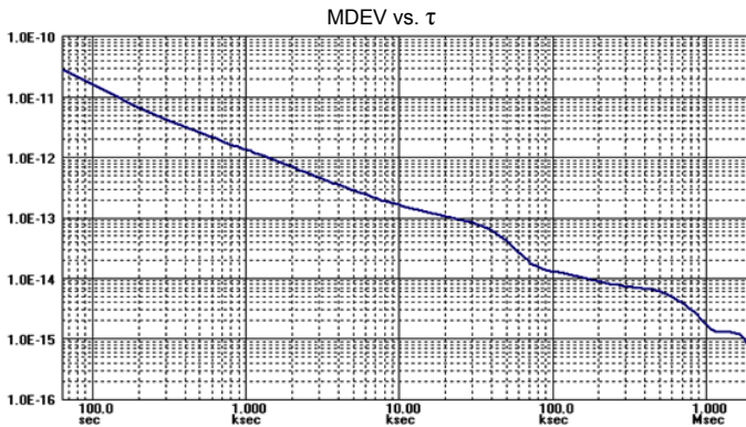
Fig. 14. The Modified Allan Deviation of the data in Fig. 13. This shows that the capability of frequency transfer approaches 1 part in 10^{15} at an averaging interval of 10 days.
