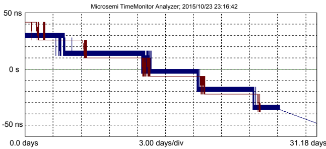
Fig. 8. PTP over OTN data with the shows a slope of -3 ns/day over a 31-day period in both forward and reverse directions.
