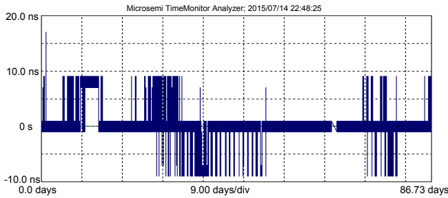
Fig. 13. A long-term run of 87 days between NIST and the AMC. The peak variation is 26 ns, showing that this method is capable of maintaining time transfer well below 100 ns.
