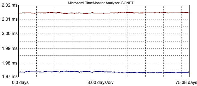
Fig. 2. PTP over SONET results over 75 days, showing the forward delay in blue and the reverse in red. The total delay is about 2\ \text{ms} with about a 40\ \mu\text{s} asymmetry.
