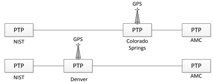
Fig. 7. Original network broken into segments by placing additional PTP equipment in Denver and in Colorado Springs.
