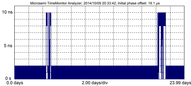
Fig. 6. Time transfer capability using the OTN. The initial phase offset of 19.1 \mu s stated in the header is due to an asymmetry of 38.2 \mu s. In the plot, the 19.1 \mu s value is subtracted in this plot. The peak-to-peak deviation is 10 ns, with the short term deviation no more than 2 ns.
