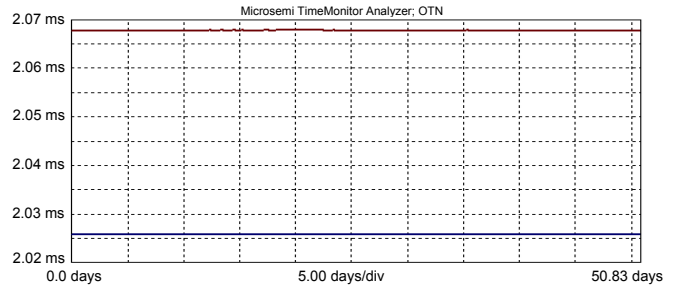
Fig. 4. PTP over OTN results over 51 days, showing the forward delay in blue and the reverse in red. As for the SONET case, the total delay is about 2\ \text{ms} with about a 40\ \mu\text{s} asymmetry.
