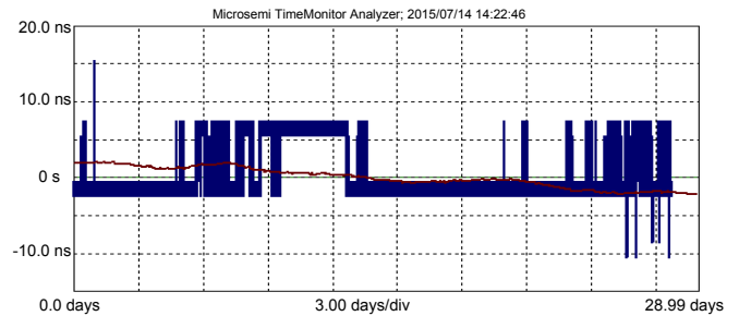
Fig. 11. A comparison of PTP fiber time transfer with GPS carrier-phase. The PTP data are in blue, the GPS data are in red. It appears that these particular PTP data do not have the precision to see the small changes between UTC(NIST) and UTC(USNO).
