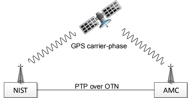
Fig. 10. Diagram depicting simultaneous time transfer measurements made using GPS carrier-phase and over fiber using PTP over OTN.
