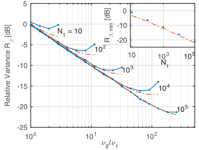
FIG. 2. Noise reduction for a frequency ratio measurement of a many-atom clock with a single-atom clock. Precise laser phase measurements on clock 1 allow the unambiguous determination of the clock 2 phase for probe durations longer than the laser coherence limit, giving a reduction of measurement noise compared to the projection noise limit for asynchronous clock comparisons with otherwise identical noise. Simulation results (points) reproduce the analytical estimates (dash-dotted lines) up to the point that the projection noise for the two clocks is comparable. Inset: Minimum relative variance R_{\beta, \text{min}} plotted vs N_1 , showing that higher atom numbers support greater suppression of the noise.
