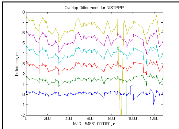
Figure 2. Overlap differences for the current NIST primary GPS receiver, for MJD's 54861-56142, successive sigma pseudoranges offset by integers.
