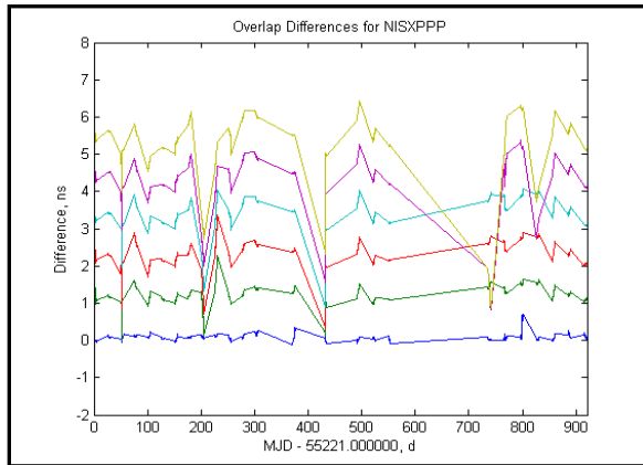
Figure 4. Overlap differences for the NISX receiver, of the same model and make as NIST , over MJD's 55221-56142, successive sigma pseudoranges offset by integers.
