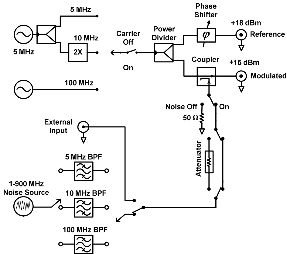
Figure 2. Block diagram of 510100 PM/AM noise standard, which selects one of three frequencies of 5 MHz, 10 MHz, and 100 MHz. BPF is the bandpass filter
