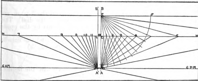
FIGURE 1.—Graphical construction for horizontal sundial
