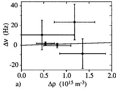
Fig. 10. Measurement of the density-dependent frequency shift (a) using cold atoms ( T \approx 3 mK), (b) using ultracold atoms ( T \approx 20 \mu K). The lines represent a linear regression to the data.
