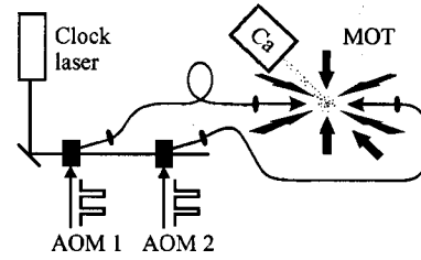
Fig. 2. Sketch of the MOT and spectroscopy setup.
