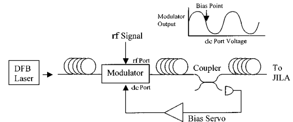
Fig. 2. Schematic of the rf transmission system from NIST to JILA. The inset shows the actively maintained dc bias point for the light power launched into the BRAN fiber.
