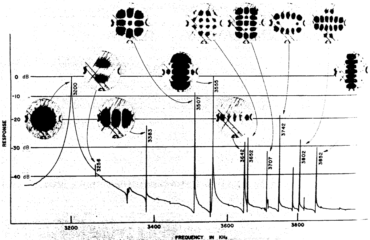
FIGURE 1. Responses and distribution of strain in contoured 3.2-MHz crystal vibrator.
