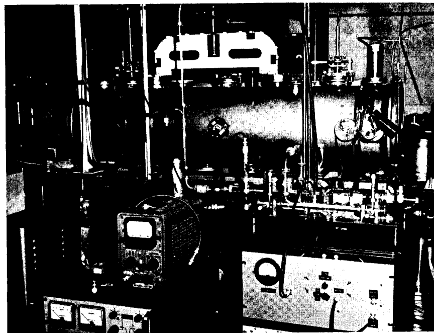
Fig. 3. The NBS thallium atomic beam frequency standard.
