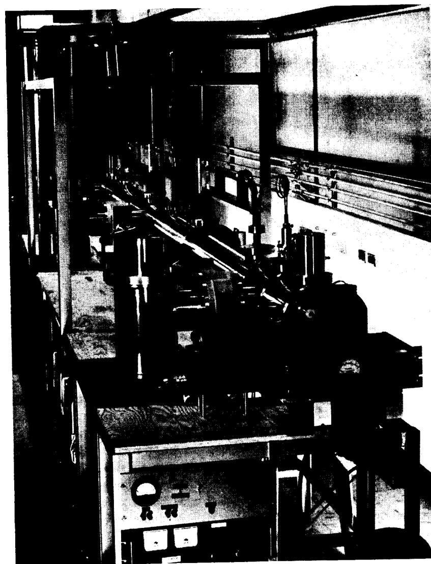
Fig. 2. Cesium atomic beam frequency standard (NBS III).
