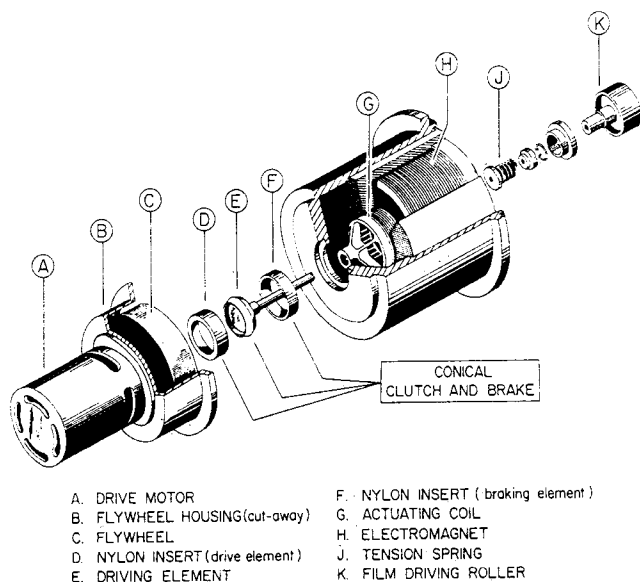
FIGURE 3. Camera mechanical drive.
