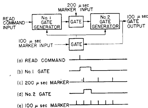
FIGURE 9. One-hundred microsecond gate generator.
