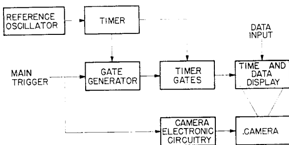
FIGURE 2. Functional system diagram.
