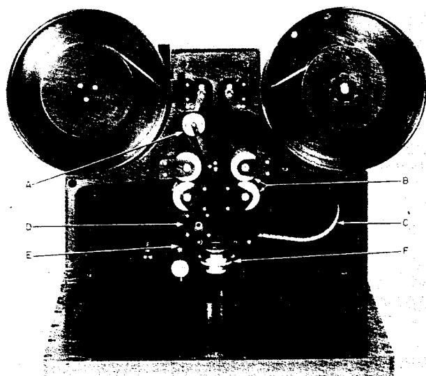
FIGURE 4. Camera interior detail.
