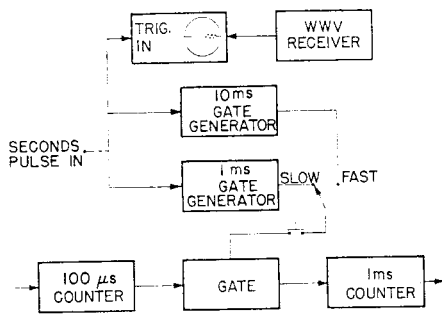
FIGURE 8. Timer synchronizing circuit.
