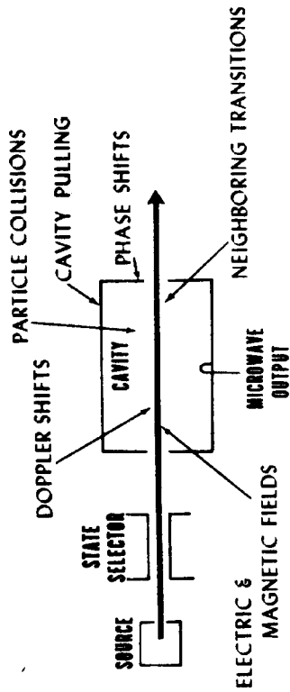
Travelling beam maser...
