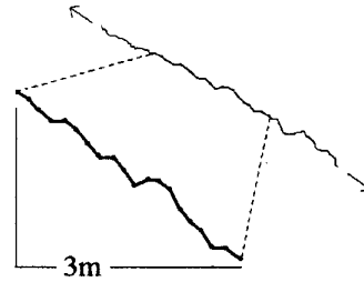
Figure 3. Procedure for TotalMod- \sigma_y(\tau) , Total- \sigma_x(\tau) , and Total- H\sigma_y(\tau) starts with original data subsequence.
